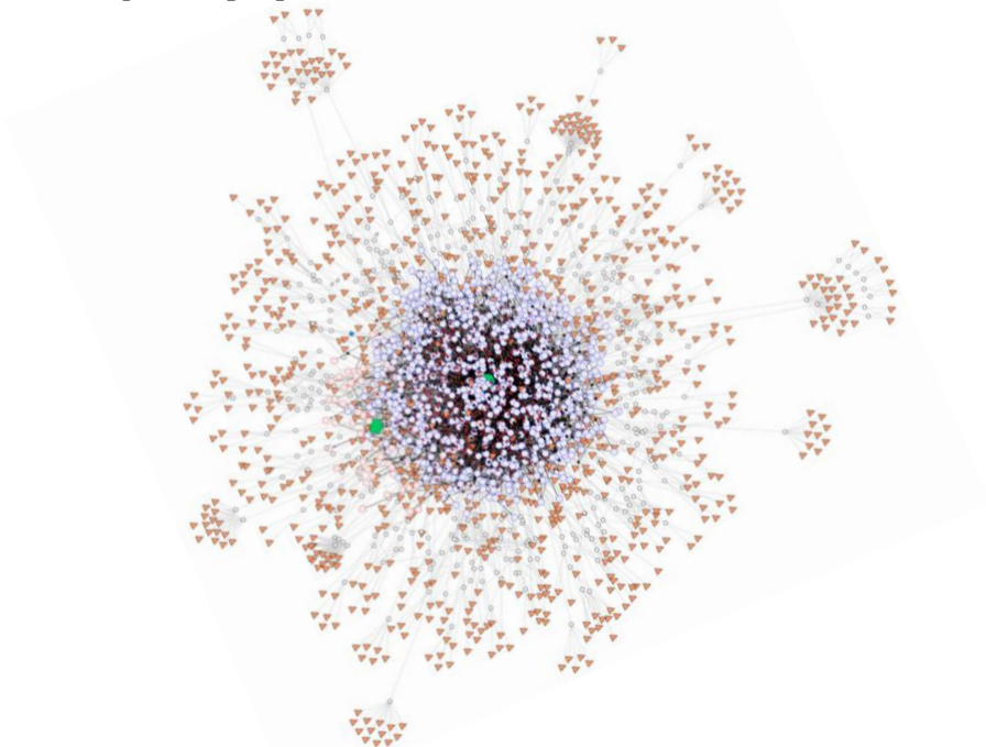
Fig. 19: Genome-scale network of C. beijerinckii NCIMB 8052 [76]
