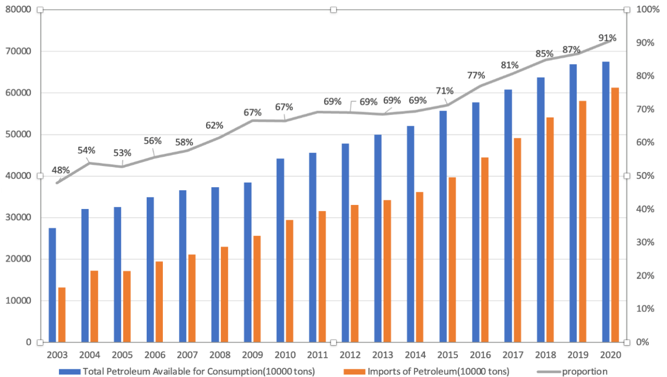
Figure 7 Total Consumption of Petroleum (10000 tons of SCE) 10
