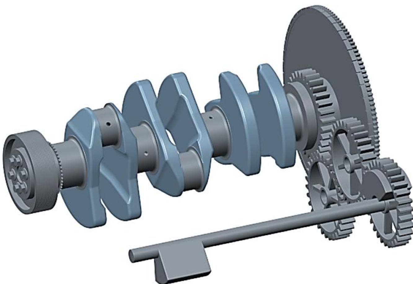
Obr. 35 Model sestavy.
