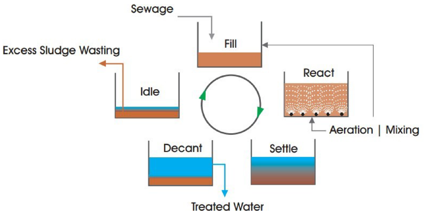
Figure 7 Sequencing batch reactors (SBR)
