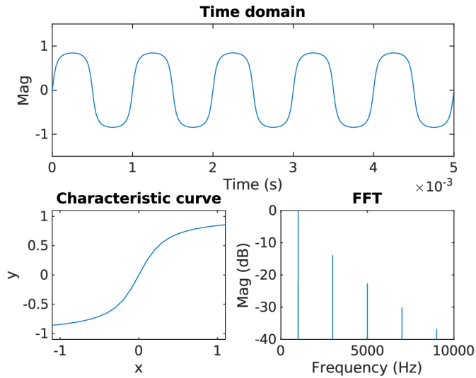
Fig. 1.6: Tape simulation for g = 4
