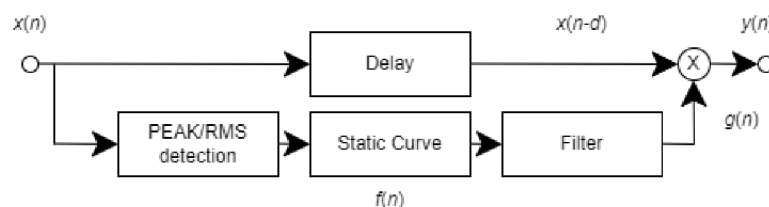
Fig. 1.7: Dynamics processing diagram (redrawn from [3], p. 106)
