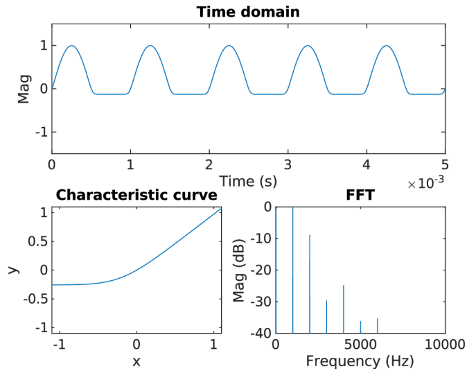
Fig. 1.5: Tube simulation for Q = -0.2 , d = 8
