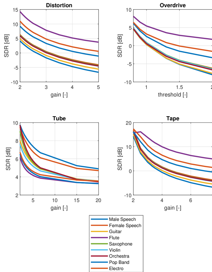
Fig. 4.1: SDR of clipped samples in relation with function parameters
