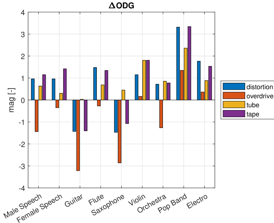
Fig. 4.5: \Delta ODG improvement of reconstructed samples
