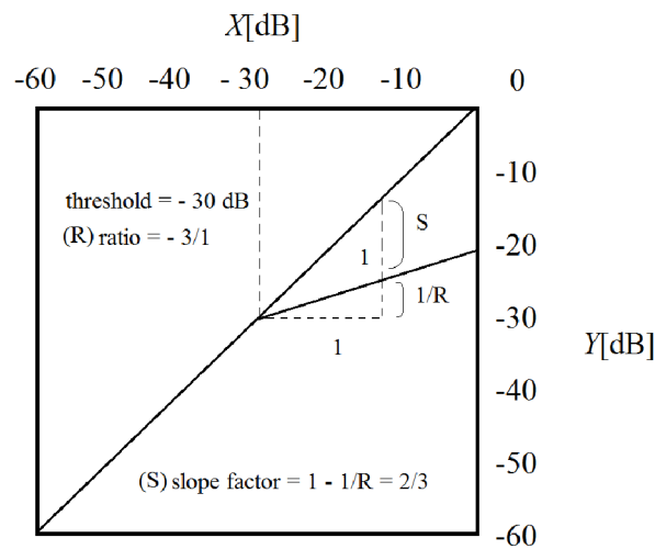
Fig. 1.8: Static characteristic of a compressor (redrawn from [3], p. 108)
