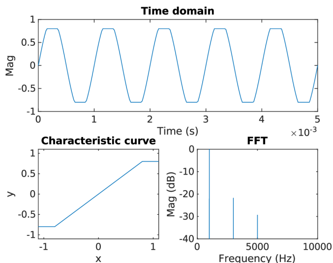
Fig. 1.2: Representation of the hard clipped signal, \theta = 0.8
