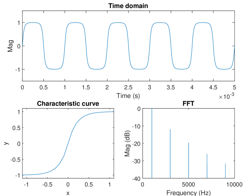
Fig. 1.3: Distortion effect for g = 4
