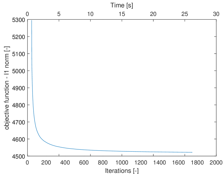
Fig. 4.2: \ell_1 norm in time/iterations
