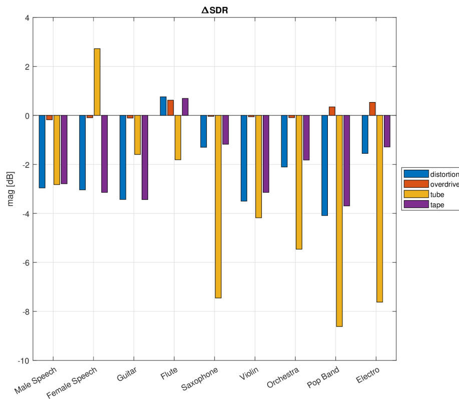
Fig. 4.4: \Delta SDR evaluation of reconstructed samples
