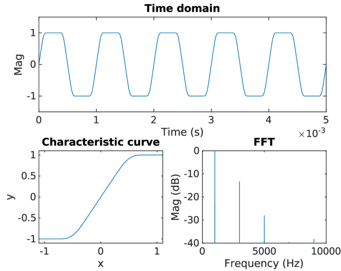
Fig. 1.4: Overdrive effect for g = 1
