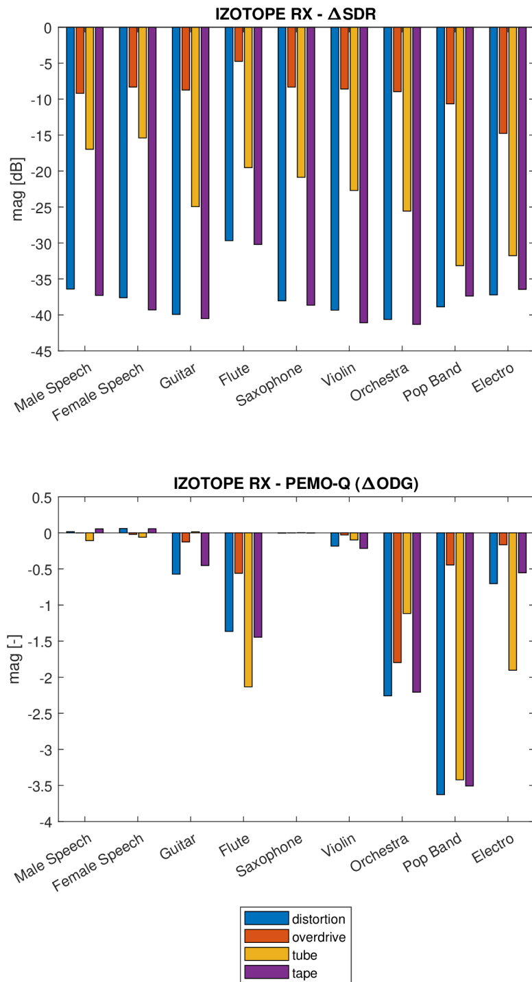
Fig. 4.8: DeClip restoration evaluation using \Delta SDR and \Delta ODG
