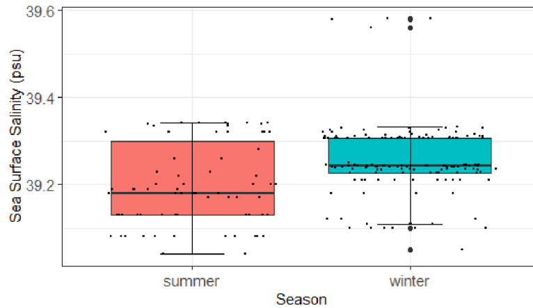
Figure 25. Sea surface salinity of photo-identified bottlenose dolphins compared to the seasons (summer and winter 2015-2021). Boxplot shows minimum value in the data, interquartile range (25th percentile, median, 75th percentile), maximum value in the data and outliers.
