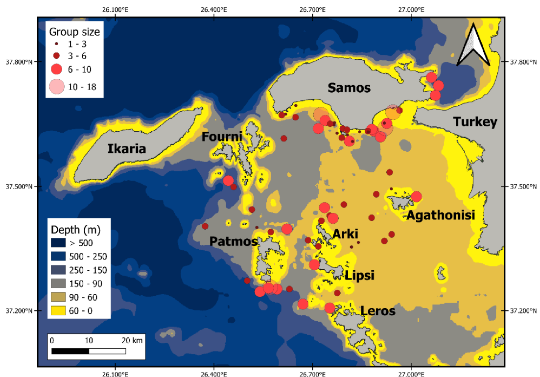
Figure 27. Group size of photo-identified bottlenose dolphins in the eastern Aegean Sea (2015-2021). The size of the circles symbolizes the number of dolphins in the group.
