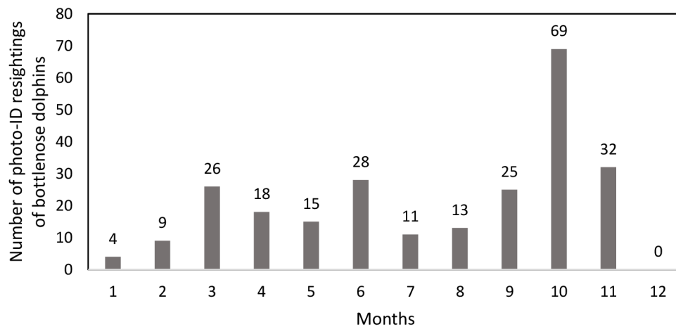
Figure 18. The number of bottlenose dolphins re-identified over the months (2015-2021).
