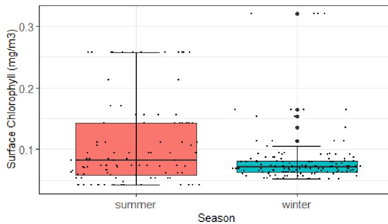
Figure 26. Sea surface chlorophyll of photo-identified bottlenose dolphins compared to the seasons (summer and winter 2015-2021). Boxplot shows minimum value in the data, interquartile range (25th percentile, median, 75th percentile), maximum value in the data and outliers.
