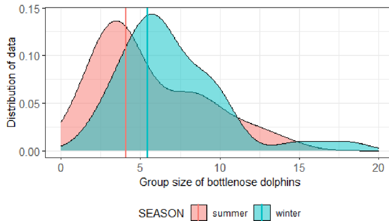
Figure 29. The density of group size (n=66) between seasons (summer and winter 2015-2021). The vertical lines demonstrate the mean value between the summer and winter seasons.
