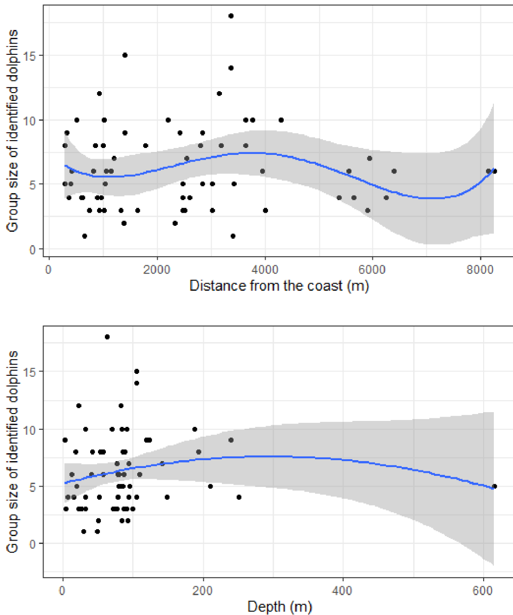
Figure 30. Effect of distance from the coast (a) and depth (b) on group size with 95% CI, (n = 66) of identified bottlenose dolphins (black circles).
