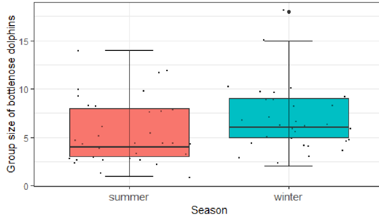
Figure 28. Group size distribution (n=66) of identified bottlenose dolphins between seasons (summer and winter 2015-2021). Boxplot shows minimum value in the data, interquartile range (25th percentile, median, 75th percentile), maximum value in the data and outliers.
