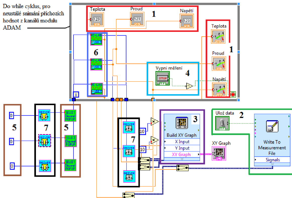
Obr. 4.2: Block Diagram
