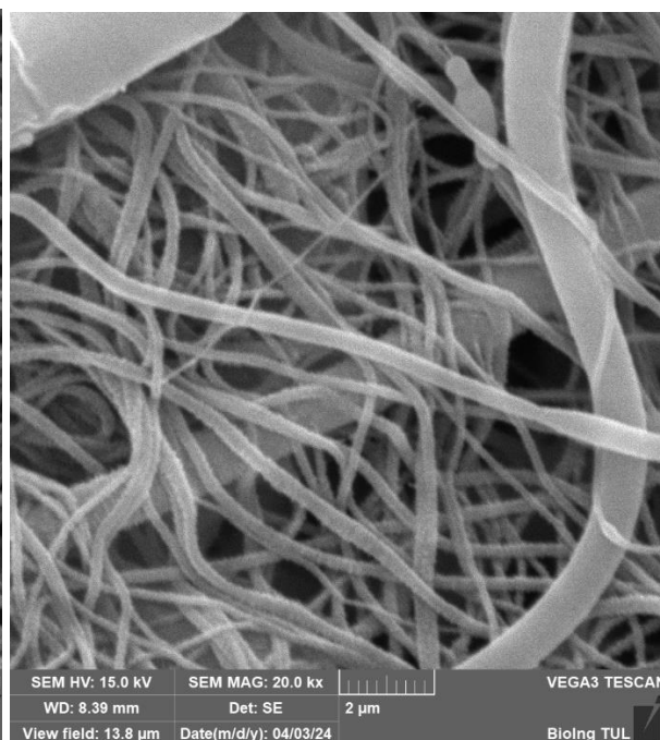
2 rub shish-kebab PCL 45
