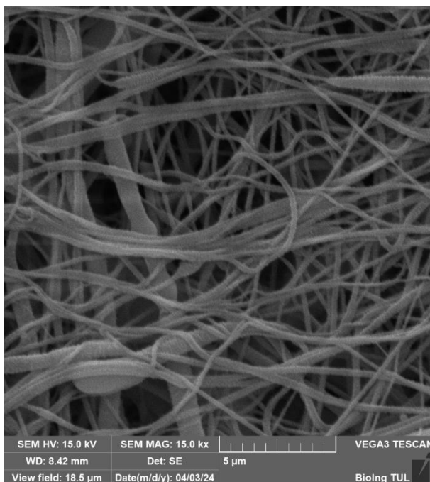
2 líc shish-kebab PCL 45
