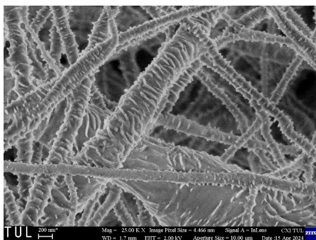
2 líc shish-kebab PCL 45
