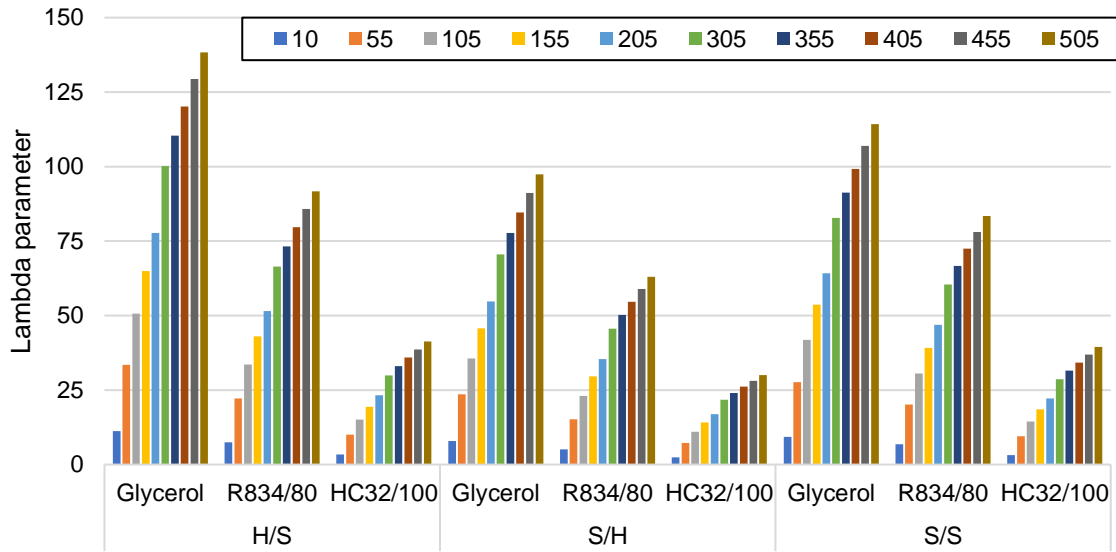
Fig. 13-10 Lambda parameters plotted for different configurations and lubricants at different speeds for fixed ball speed using Nijenbanning equation.
