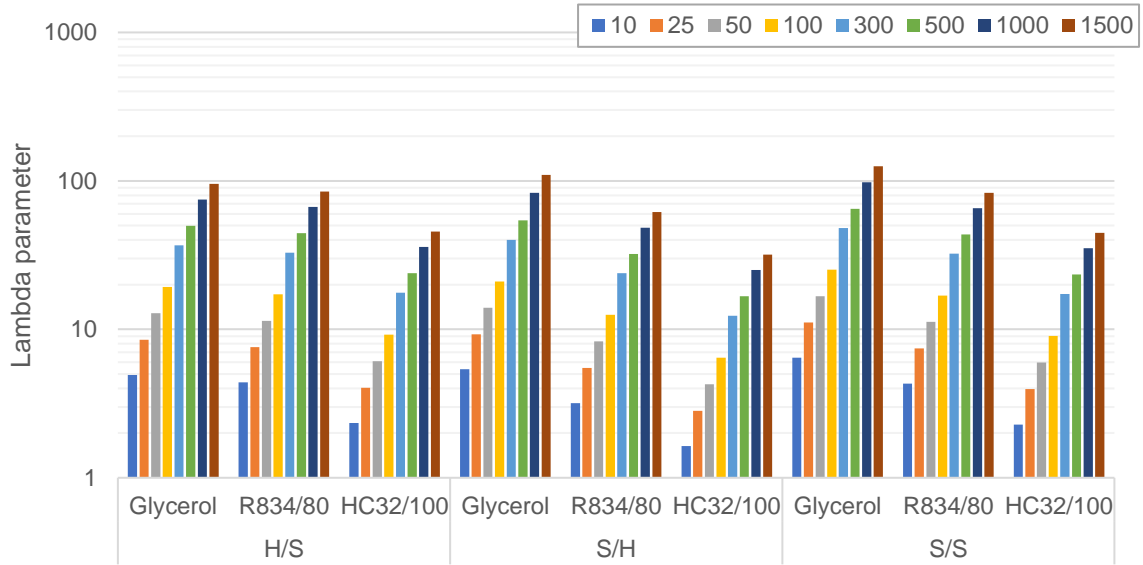
Fig. 13-3 Lambda parameters plotted for different configurations and lubricants at different speeds for SRR = 150 % using Nijebanning equation.
