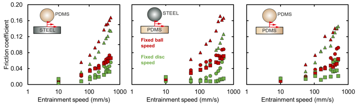
Fig. 5-33 Friction coefficient plotted as a function of log-entrainment speed for the fixed ball speed and the fixed disc speed scenarios for all configurations.
