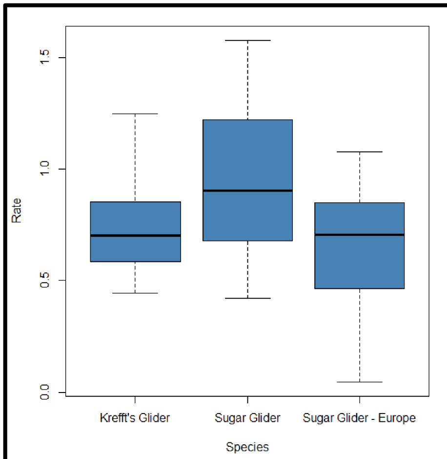
Figure 9: The boxplot graph demonstrating the differences among groups in the Rate parameter.
