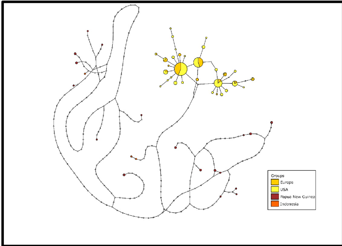
Figure 8: TCS haplotype network using ND2 gene including 76 sequences from Europe, 140 from the USA (Campbell et al. 2019), and 29 sequences from Indonesia and Papua New Guinea (Malekian et al. 2010). The circles represent haplotypes and are proportional to their frequency. Mutation steps are visualized with empty circles. Color codes of the circles represent the origin of the sequences.
