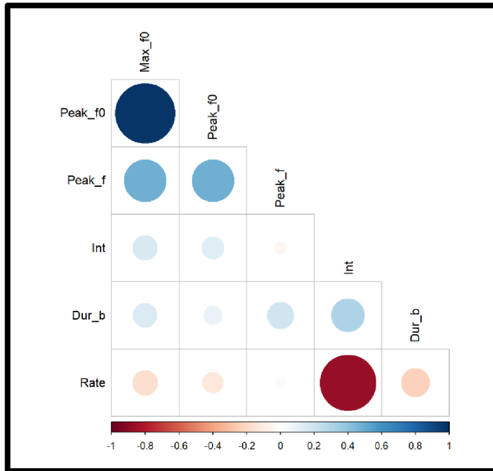
Figure 10: Correlation of the measured acoustic parameters.
