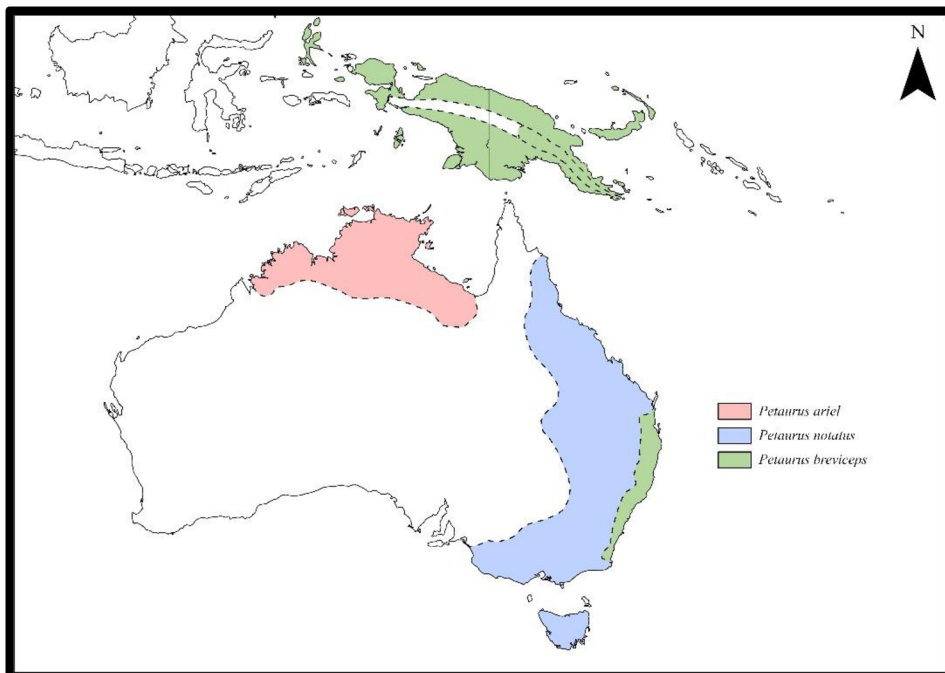
Figure 2: Proposed distribution of Petaurus breviceps together with new Australian species (Smith 1973; Cremona et al. 2021). The map was redrawn in the ArcGIS Pro 3.0.2 software (Esri 2022, 2023).
