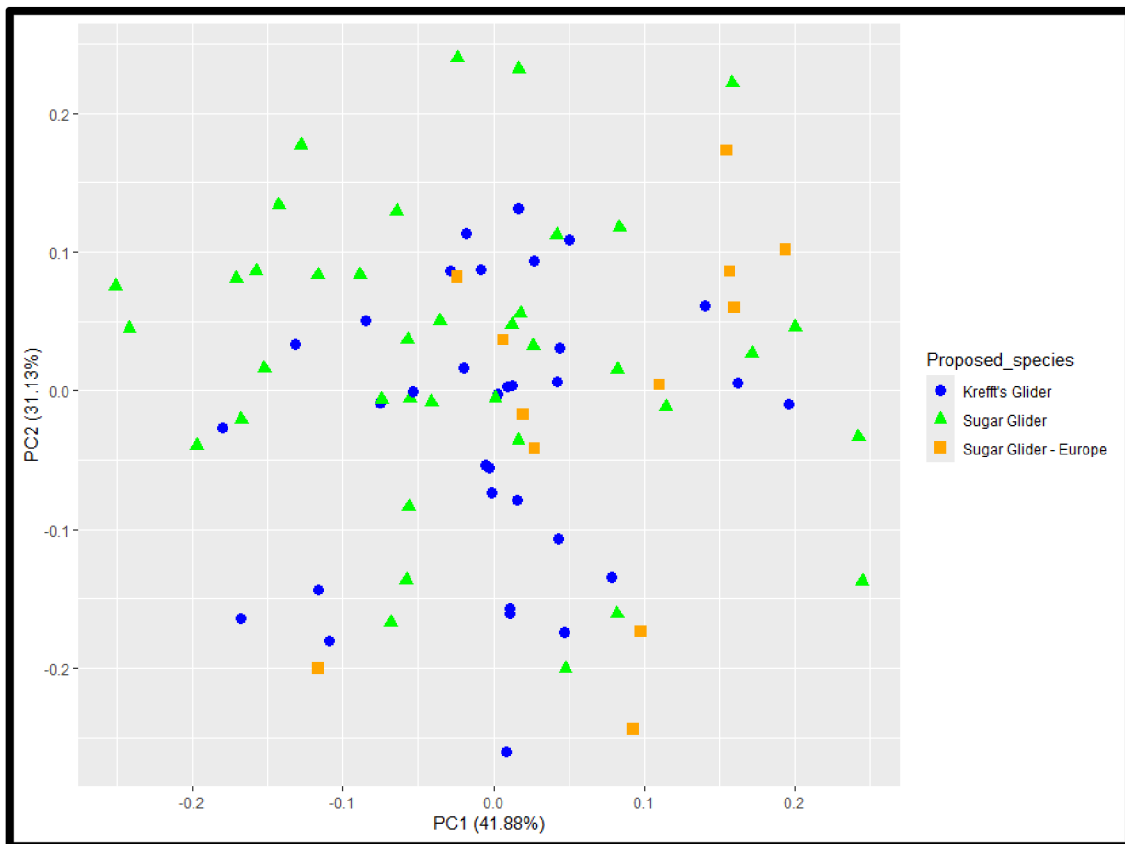
Figure 11: Scatterplot showing the position of each call within the dimension of the two principal components.
