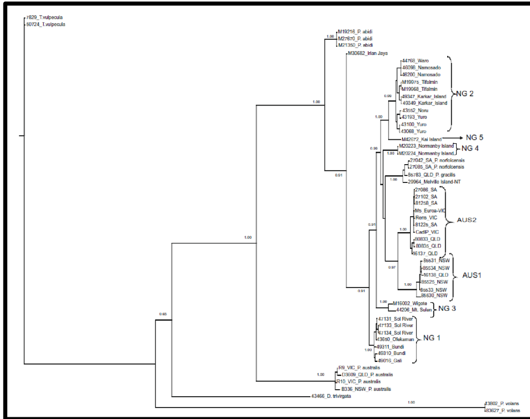
Figure 1: Bayesian consensus tree demonstrating the phylogenetic relationships of Petaurus breviceps s.l. and other Petaurus species, which are indicated on the label (Malekian et al. 2010).
