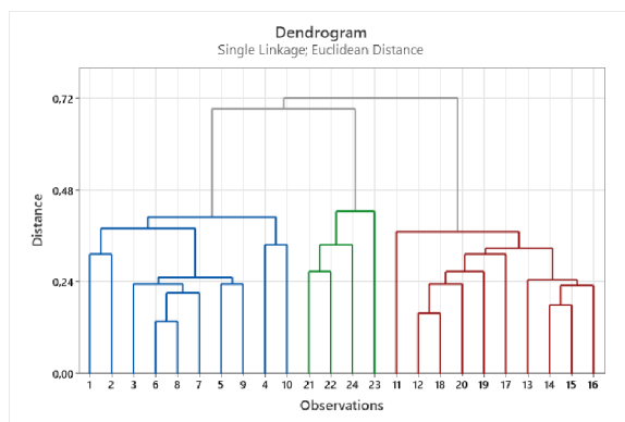
(a) Dendrogram 4
