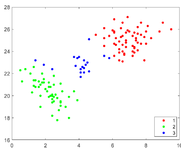
(b) K-means 2
