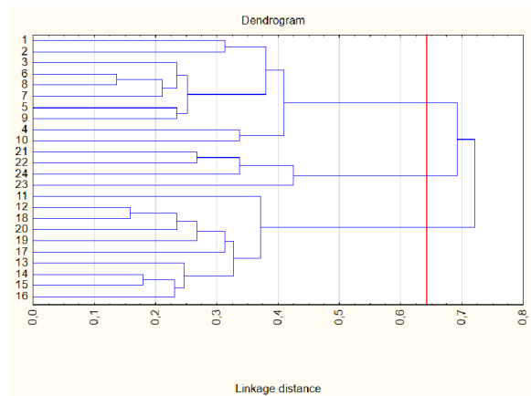
(b) Dendrogram 4
