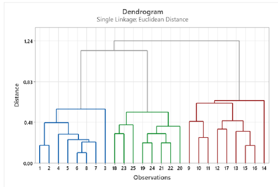
(a) Dendrogram 3
