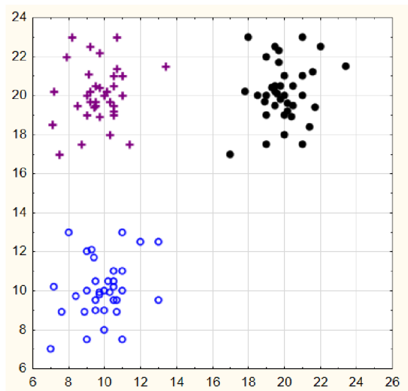
(a) K-means 1
