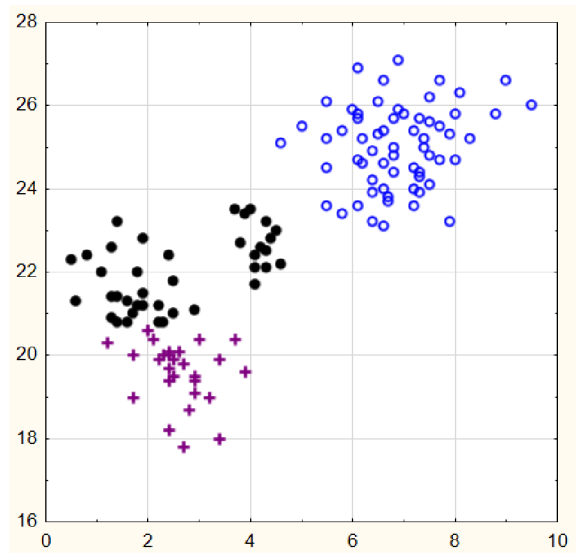
(b) K-means 2
