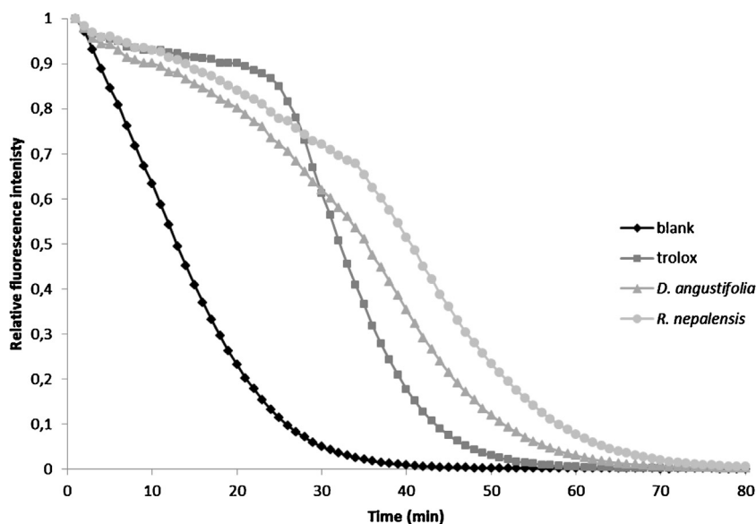
Fig. 2. Kinetic curves of fluorescein decay induced by AAPH radical in the presence of Dodonaea angustifolia and Rumex nepalensis (roots) extracts at concentration of 1 µg/mL in comparison to positive (trolox) and negative (blank) controls (ORAC assay).
