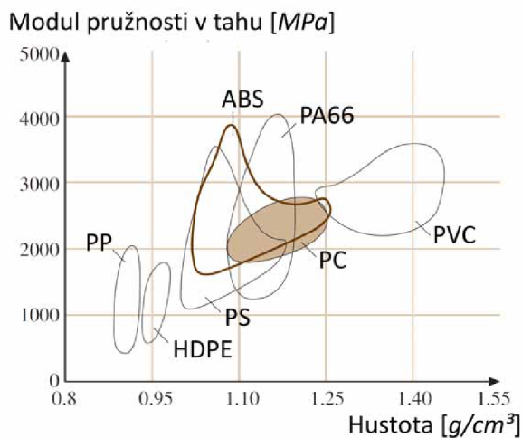
Obr. 3.13 El. modul vs. hustota [25]
