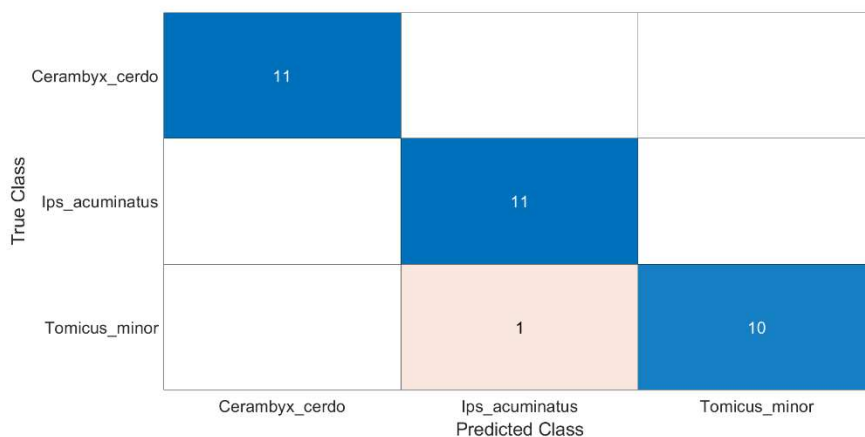
Fig. 21 - Grid division method, confusion matrix - 3 classes
