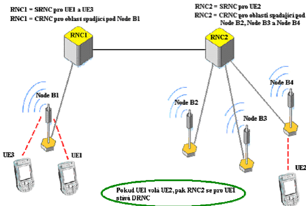
Obr. 2.8: Role RNC
