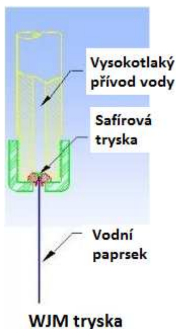
Obr. 1.31 WJM tryska [6]
