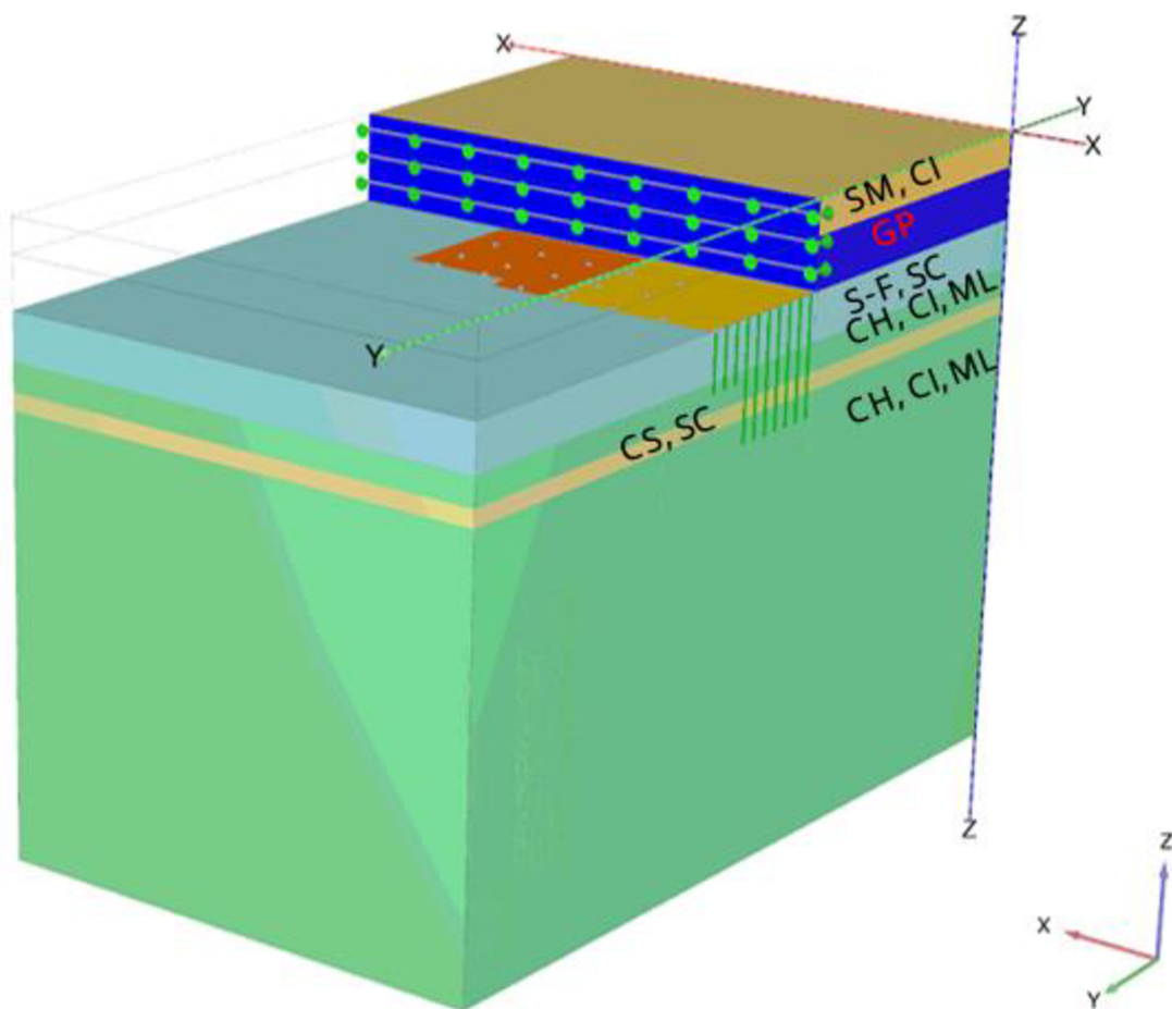
Obr. 5-4: Geometrie modelu
