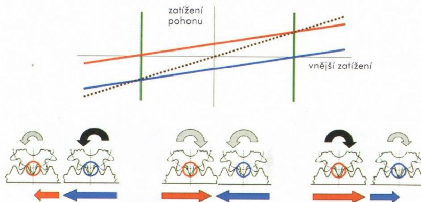
Obr. 28) Master-Slave princip [1]
