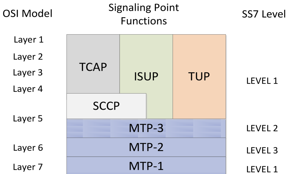
Figure 2 - SS7 protocol stack.
