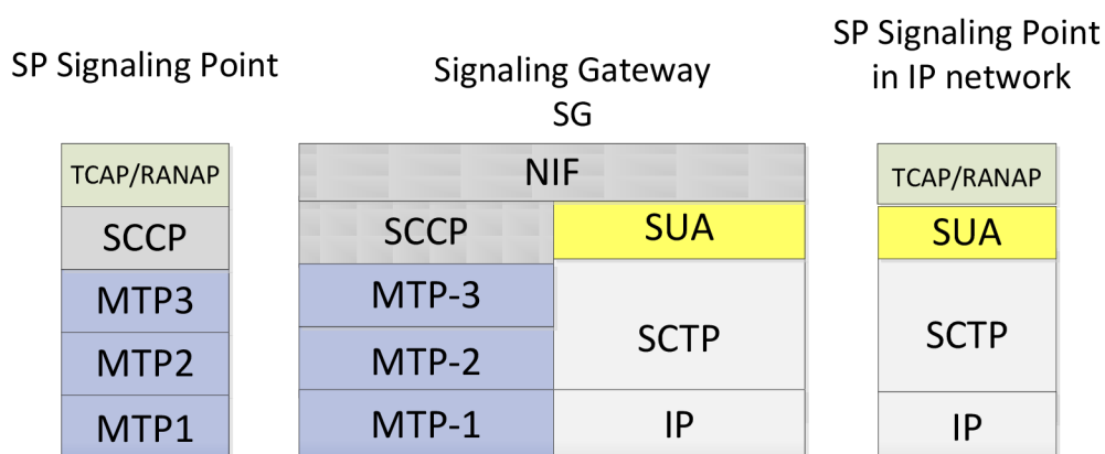
Figure 13 - SUA - structure for connectionless transmission
