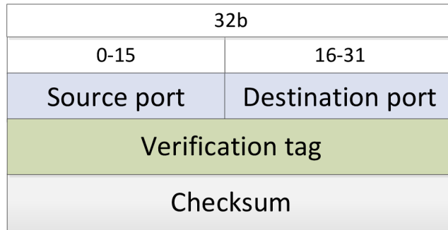
Figure 9 - SCTP Header Format
