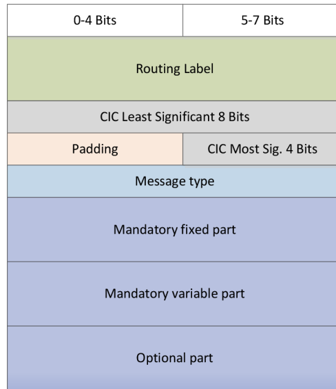
Figure 5 - ISUP message format
