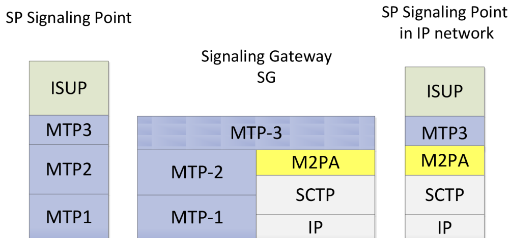
Figure 10 - Communication using M2PA protocol
