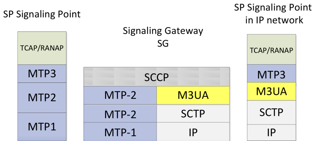
Figure 12 - Communication using M3UA protocol
