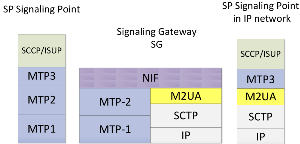
Figure 11 - Communication Protocol using M2UA
