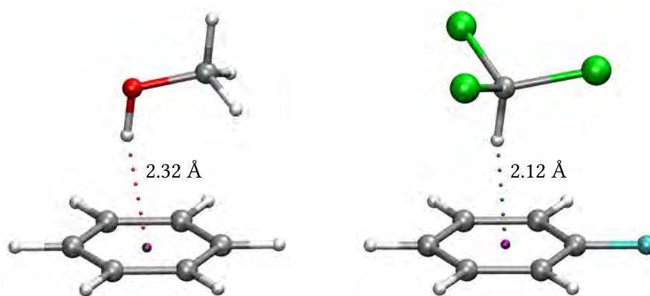
Figure 2.3: Hydrogen bonded complexes showing R-H\cdots\pi interaction. On the left is complex of methanol with benzene. Its measured experimental IR shift of O-H stretching frequency is -14\text{ cm}^{-1} 17 . On the right is blueshifting complex of chloroform and monofluorobenzene with respective shift of C-H stretching frequency by 14\text{ cm}^{-1} 15 .
