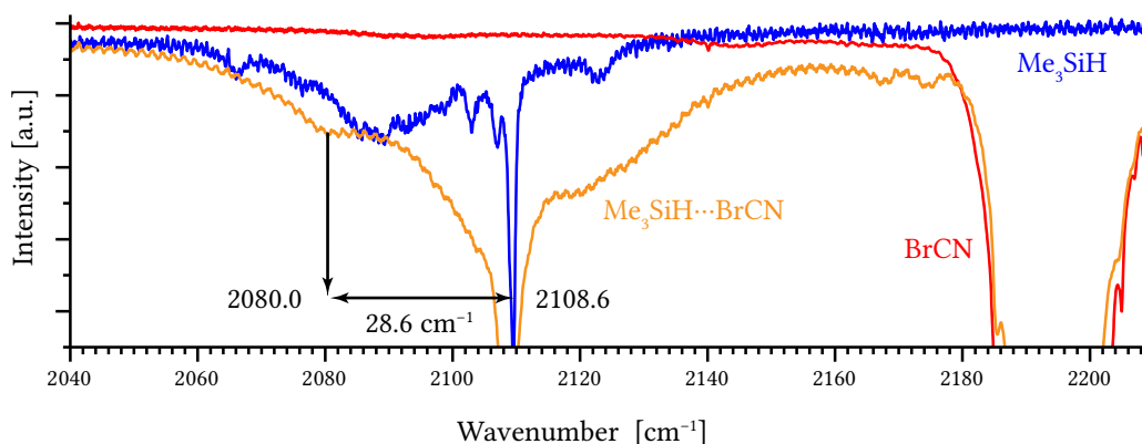
Figure 5.4: Ar-matrix spectra of the \text{Me}_3\text{SiH}\cdots\text{BrCN} complex.
