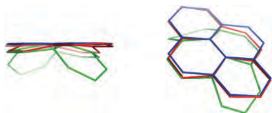
Fig. 7 Comparison of planar pyrene (blue) and pyrene motifs cut from carbon nanotube (red) and C-site of C_{70} (green) viewed from different angles.
