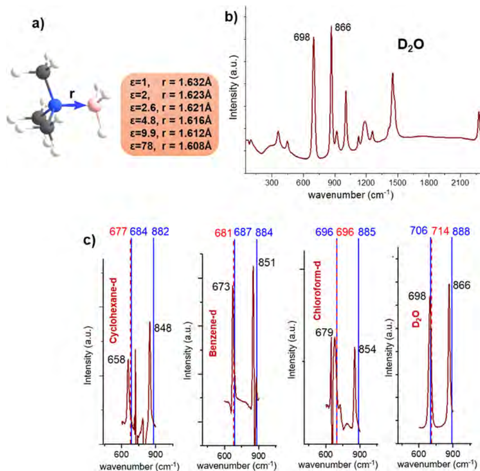
Fig. 1 The calculated and observed structural and spectroscopic data of Me 3 NBH 3 . a The optimized geometry of Me 3 NBH 3 . The B–N distances ( r ) are given in the gas phase ( \epsilon = 1 ) and various solvents, cyclohexane ( \epsilon = 2.0 ), carbon disulfide ( \epsilon = 2.6 ), chloroform ( \epsilon = 4.8 ), o -dichlorobenzene ( \epsilon = 9.9 ), and water ( \epsilon = 78.0 ); b the Raman spectra of Me 3 NBH 3 measured in D 2 O; c the relevant part of the Raman spectra ranging 450–1050 cm -1 in various solvents. The PBE0-D3/def2-QZVP calculated harmonic (in blue color) and anharmonic (in red color) frequencies are shown (C: gray, N: blue, H: white, B: pink).
