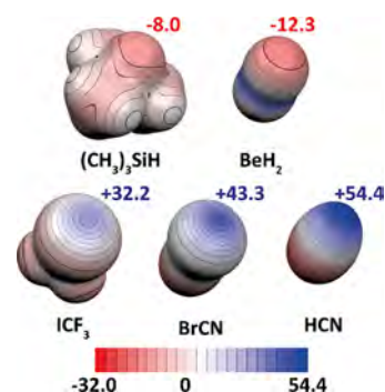
Figure 5. MEP calculated at the \omega\text{B97X-D/def2-QZVPP} level for the monomers studied. The ESP scale is in kcal/mol. The V_{s,\text{max}} on the hydrogen atom from the \text{Me}_3\text{SiH} molecule is depicted in red. The V_{s,\text{min}} in the center of the \sigma -hole or on top of the hydrogen atom is in blue.
