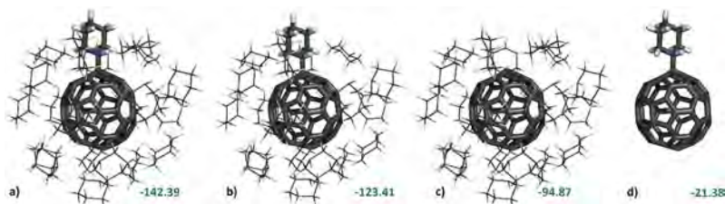
Figure 2. PBE0-D3/6-31G(d) interaction energies of the complexes C_{60} \cdots (C_5H_{11}N)_{21} (a), C_{60} \cdots (C_5H_{11}N)_{20} (b) with dative bond, C_{60} \cdots (C_5H_{11}N)_{20} (c) without dative bond and C_{60} \cdots C_5H_{11}N (d). The geometries of C_{60} \cdots (C_5H_{11}N)_{20} and C_{60} \cdots C_5H_{11}N are extracted from the PBE0-D3/6-31G(d) optimized geometries of C_{60} \cdots (C_5H_{11}N)_{21} .
