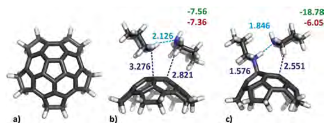
Figure 6. PBE0-D3/def2-TZVPP optimized geometries of C 30 H 20 with selected hydrogen bond lengths between pips (light blue) in Å, and ΔE INTR (green) and EA (red) in kcal mol –1 .
