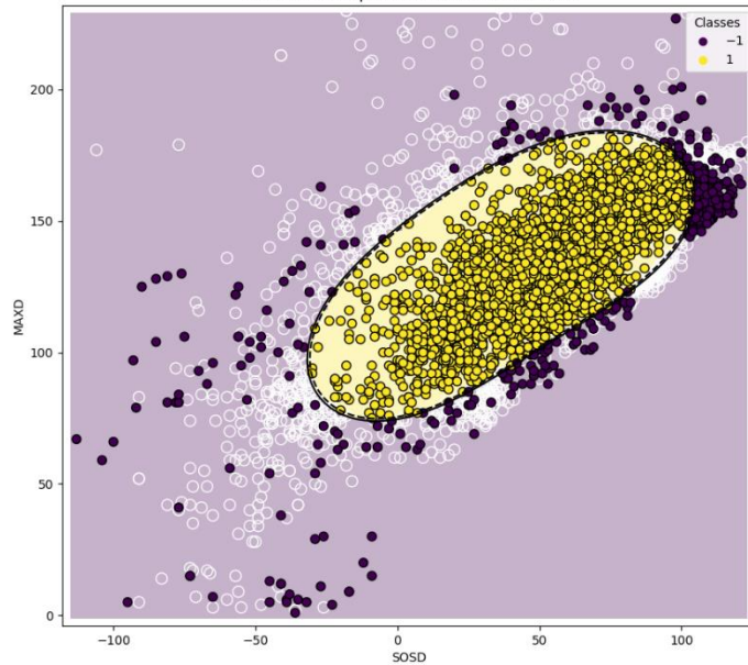
Decision boundaries of rbf kernel in OCSVC using {'gamma': 'scale', 'kernel': 'rbf', 'nu': 0.16} on 2019 data. The number of predicted dead trees is: 3825
