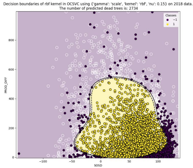
Figure A1. 7. Decision boundary for One-Class SVM for feature set of ['SOSD', 'PROD_DIFF'], using hyperparameters: {'gamma':'scale', 'kernel':'rbf', 'nu':0.15} on validation dataset #1 (2018). Accuracy: '1': dead tree prediction, '-1': outlier. 82.30 %
