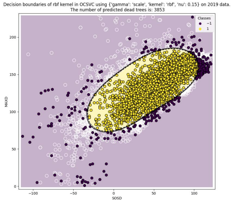
Figure 4. Decision boundary for One-Class SVM for feature set of ['SOSD', 'MAXD'], using hyperparameters: {'gamma':'scale', 'kernel':'rbf', 'nu':0.15} on validation dataset #2 (2019). '1': dead tree prediction, '-1': outlier. Accuracy: 91.32 %
