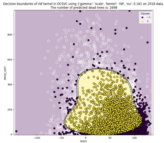
Figure A1. 8. Decision boundary for One-Class SVM for feature set of ['SOSD', 'PROD_DIFF'], using hyperparameters: {'gamma':'scale', 'kernel':'rbf', 'nu':0.16} on validation dataset #1 (2018). '1': dead tree prediction, '-1': outlier. Accuracy: 81.22 %
