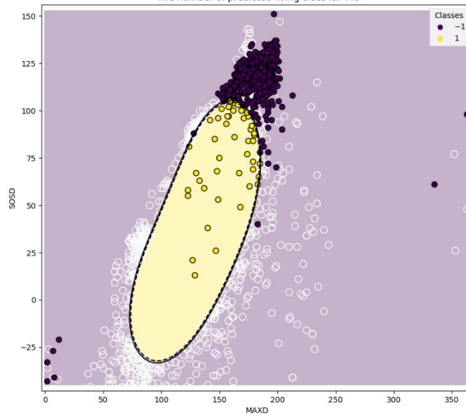
Decision boundaries of rbf kernel in OCSVC using {'gamma': 'scale', 'kernel': 'rbf', 'nu': 0.15} on living data. The number of predicted living trees is: 449
