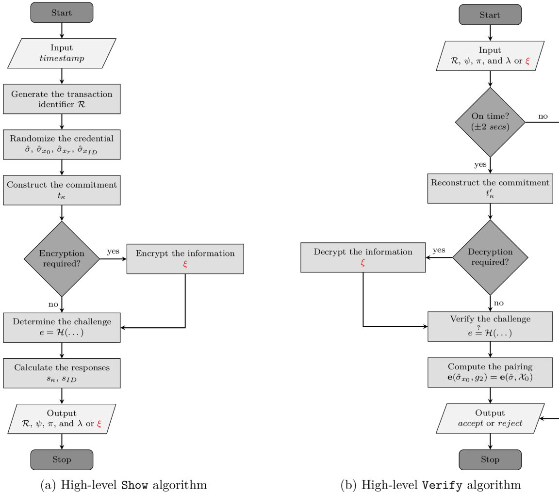
Fig. 5.2: High-level definition of the Show and Verify algorithms
