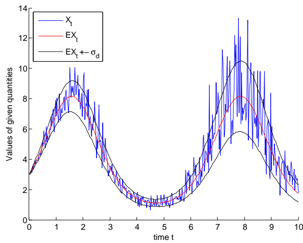
Figure 7.16: The sample path of the solution X_t fitted with its expectation and EX_t \pm \sigma_d
