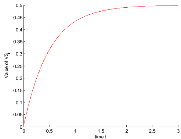
Figure 7.4: The variance of S_t
