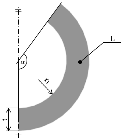
Obr. 8.2 Model geometrie
