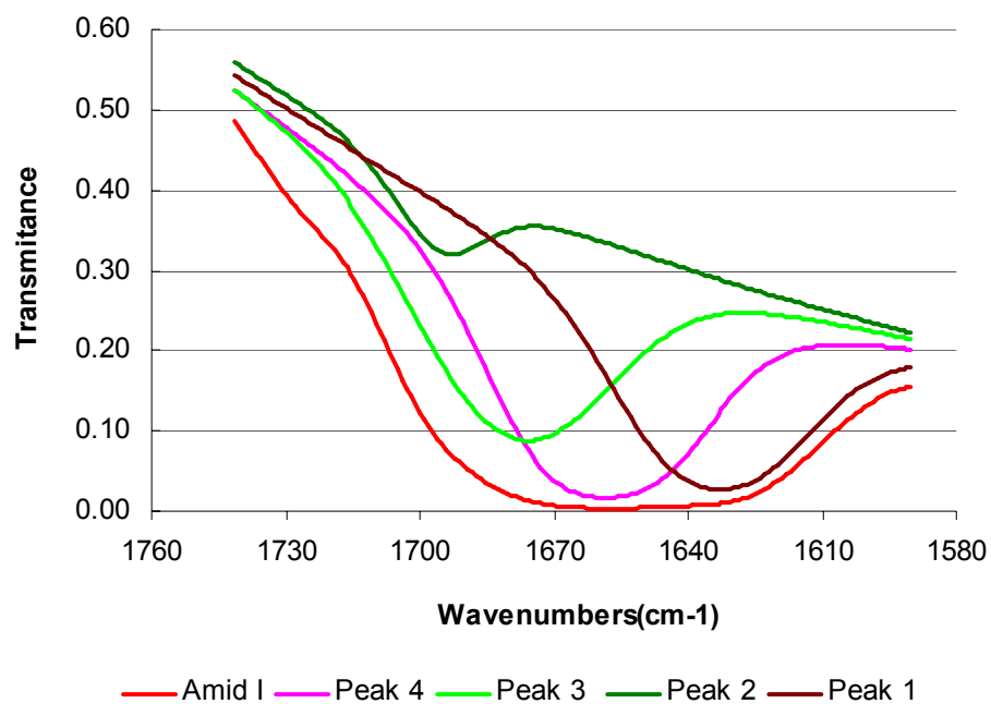
A 9 Amid I band of pure collagen/cellulose mixtures in ratio of 1:9 with fitted components.
