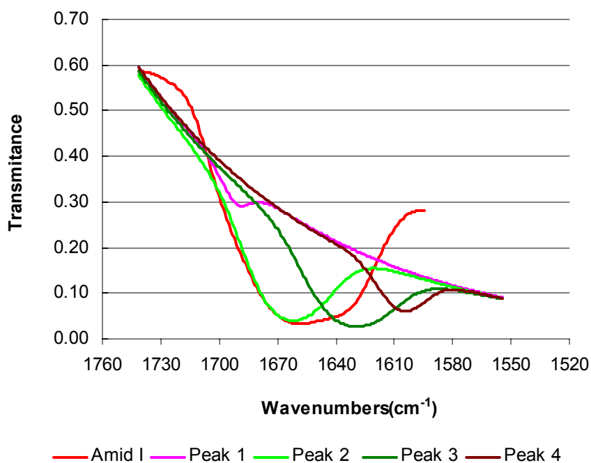
A 23 Amide I band of activated collagen/cellulose mixtures in the film in the ratio of 9:1 with fitted components.
