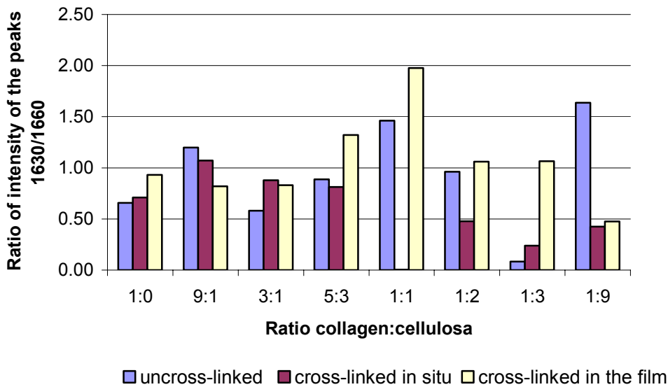
Figure 48 The dependence of intensity peaks 1630/1660 ratio on collagen/cellulosa ratio.
