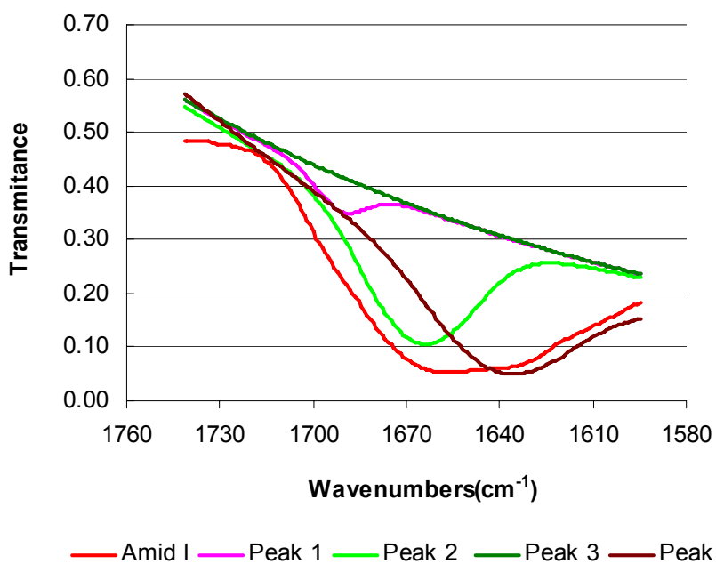
A 27 Amide I band of activated collagen/cellulose mixtures in the film in the ratio of 1:2 with fitted components.
