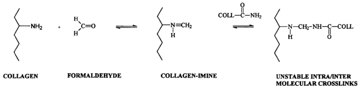
Figure 5 Formaldehyde reactions with amino groups on collagen to form cross-links [16].
