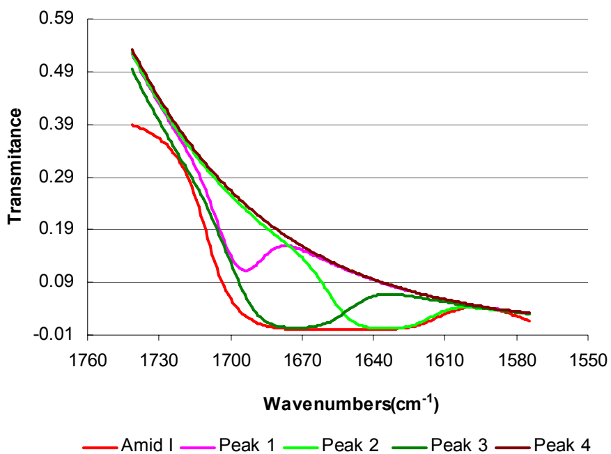
A 22 Amide I band of activated collagen/cellulose mixtures in the film in the ratio of 1:0 with fitted components.
