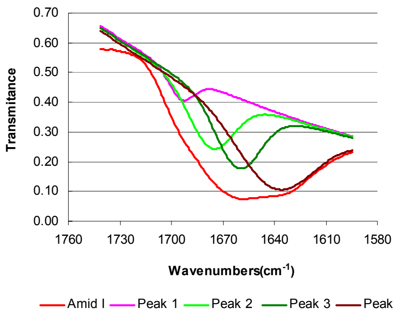
A 26 Amide I band of activated collagen/cellulose mixtures in the film in the ratio of 1:1 with fitted components.
