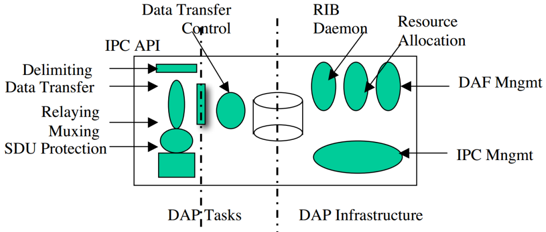
Figure 2.1: IPC Process scheme [6]
