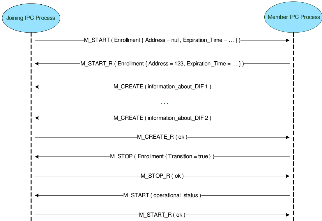
Figure 5.1: Enrollment communication when IPC Process is joining a DIF for the first time
