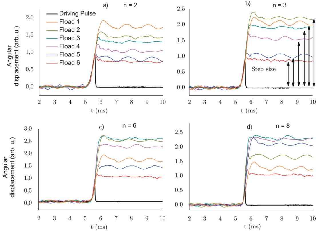
Fig. 2.7: Actuator response expressed by the PSD signal (proportional to the angular rotor displacement) to the single driving pulses (black curves) with f = 94 Hz and \tau = 10 ms for six incremental load forces ( F_{load 1} – the smallest force) and four driving pulses of the shapes given by the exponents (a) n = 2 , (b) n = 3 , (c) n = 6 , and (d) n = 8 .
