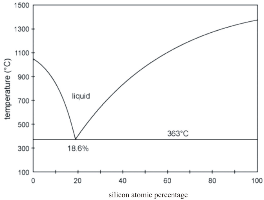
Fig. 5.26: Gold-silicon phase diagram. If a thin viscous interface layer is formed, capillary forces become significant and influence the embedding. In the viscous interface the upward flux of silica is driven by the wetting, the contact angle is in the range 0^\circ < \vartheta < 90^\circ . The flux is stopped on the triple phase line where silicon oxidizes and forms the rim. This mechanism causes a continual silica transfer from the area below the crater to the rim, until the thermodynamic equilibrium is reached.
