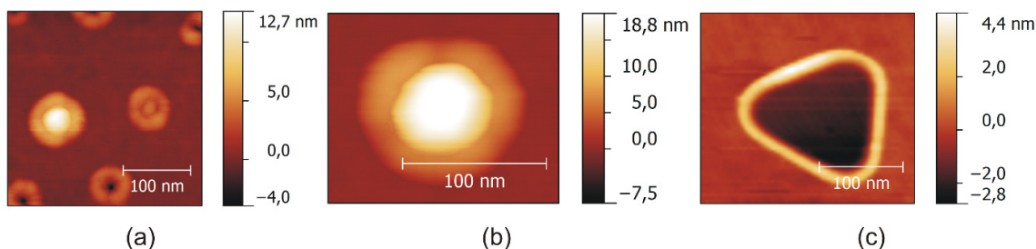
Fig. 5.2: AFM images of the modified silica surface with empty- and partially immersed in craters (a), a crater with the surrounding rim and remaining gold island inside (b), an empty crater with the surrounding rim (c).
