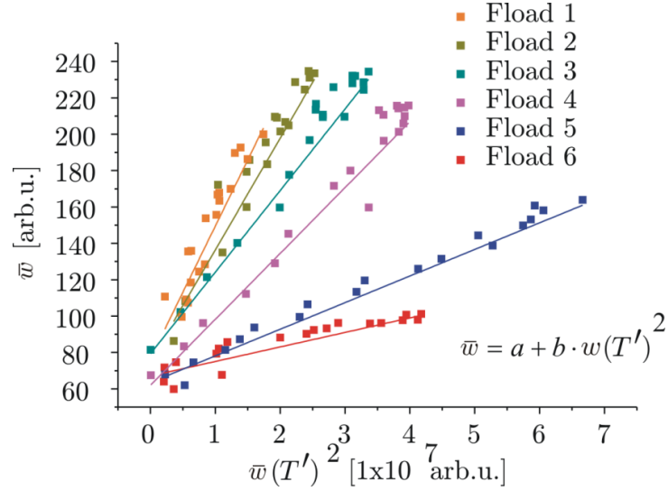
Fig. 2.9: Experimental dependence of the average angular velocity \bar{\omega} on the second power of the instantaneous angular velocity of the actuator at T' , i.e. \bar{\omega}(T')^2 , for the pulses of various exponents ( n = 1 - 10 ) and different load forces F_{load} . Repetition frequency of the pulse sequence was f = 94 Hz and pause \tau = 10 ms.
