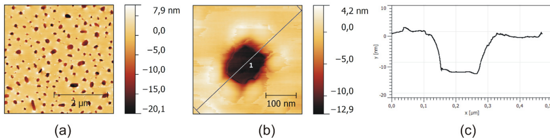
Fig. 4.2: AFM images (a, b) of the pattern prepared by annealing of a 12nm-thick gold layer at 600 °C for 10 hours. The detailed view (b) and depth profile (c) of the crater.
