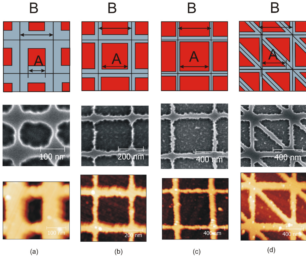
Fig. 4.10: Schematic view of different elementary units (upper row) and corresponding fabricated patterns imaged by SEM (middle row) and AFM (bottom row). The size A of the square shaped units is 100 nm (a), 300 nm (b), and 500 nm (c). The characteristic size of the right-triangle shape A is 600 nm (d).
