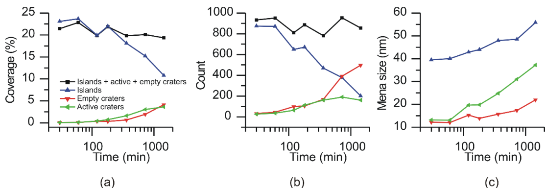
Fig. 5.10: Time evolution of surface coverage (a), counts (b) and mean lateral size (c) of the islands, craters and active craters during annealing at 1000 \text{ }^\circ\text{C} . The data were collected from the area 21.6 \mu\text{m}^2 .
