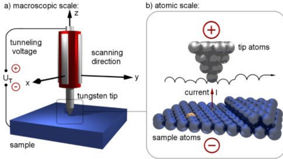
Fig. 1.1: Schematic view of a STM setup with a scanner and tungsten tip (a). View of a tip and sample at atomic scale (b).
