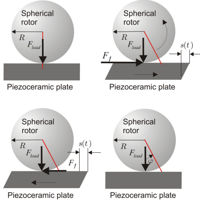
Fig. 2.5: Schematic of a 2D actuator model configuration in 4 phases during one single step: (a) initial piezo plate position, (b) piezo plate forward motion and (c) piezo plate backward motion and (d) piezoceramic plate final position ( R - rotor radius, F_{load} - load force, F_f - friction force, s(t) - piezoceramic displacement, and \varphi(t) - rotor angular displacement).
