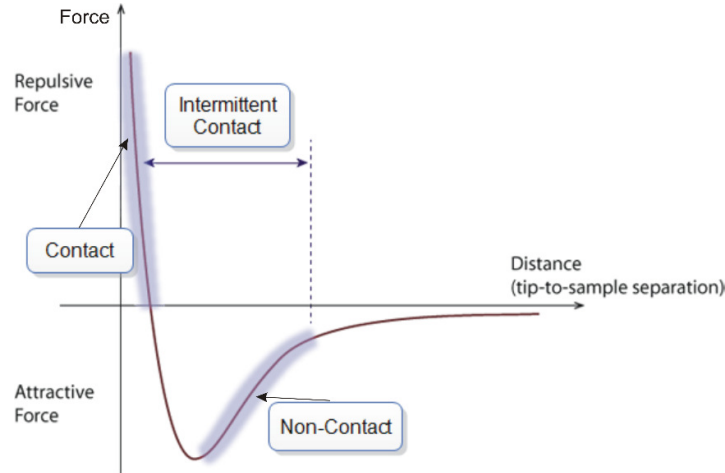
Fig. 1.3: Schematic illustration of the AFM operational modes having different working tip - sample distances.
