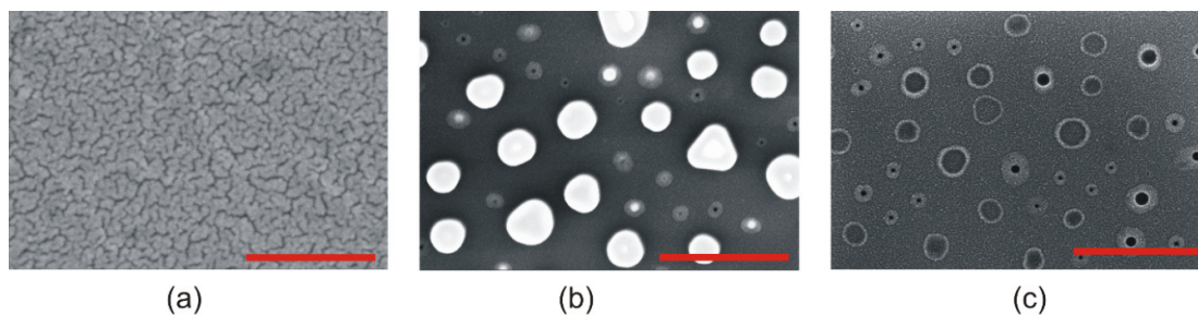
Fig. 5.1: SEM image of as a deposited 10 nm-thick gold layer on silica (a), the sample after annealing at 1000 °C for 6 hours (b) and after gold dissolution in aqua regia (c). The scale bar is 500 nm.
