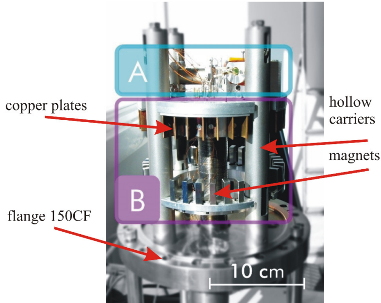
Fig. 1.5: UHV AFM/STM setup composed of a measuring head with a scanner and optical detection system (A) and anti-vibration stage with eddy current dumping (B).
