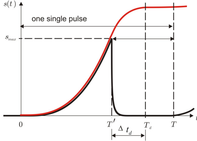
Fig. 2.6: Schematic view of the driving pulse (black) and actuator response (red) with three specific time sections defined by T' , T_d and T .
