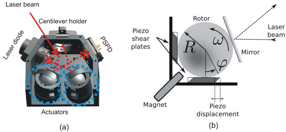
Fig. 2.1: A view of the optical detection system with a couple of the actuators used for the alignment of the laser beam with respect to the AFM cantilever and PSPD (a). Cross section of the three-axis rotary slip-stick actuator with the legend (b). For testing the actuator response the cantilever was replaced by a mirror.
