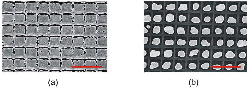
Fig. 4.18: SEM images of the 15 nm-gold thin film deposited on to the square-like patterns with a unit size of 300 nm annealed at 300 °C for 1 hour (a) and 13 hours (b). The scale bars are 1 \mu\text{m} .
