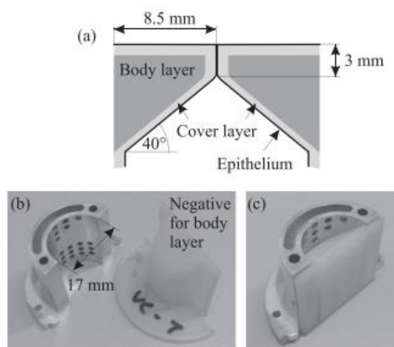
Figure 17: Central coronal cross-section through the silicone layer (a), the aluminium frame and the negative (b) and the frame and the negative glued together (c) used in fabrication of three-layer self-oscillating vocal fold model. Taken from Birkholtz et al. (2019).
