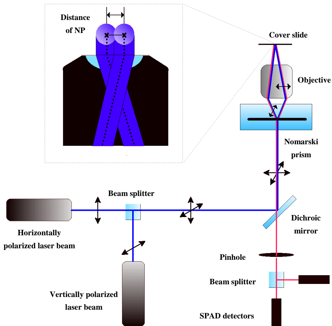
Figure 10: The optical set-up of 2f-FCS measurement.
