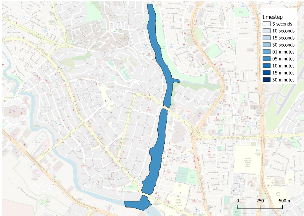
Figure E.20: Maximum water surface elevation output for a upstream boundary condition of ten-years return period hydrograph, main channel roughness = 0.066 and flood plain roughness = 0.144, and time step = 5 minutes.
