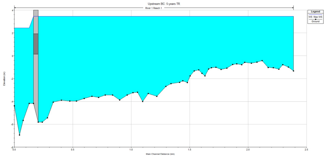
Figure E.1: Maximum water surface elevation output for an upstream boundary condition of 5-year return period hydrograph.
