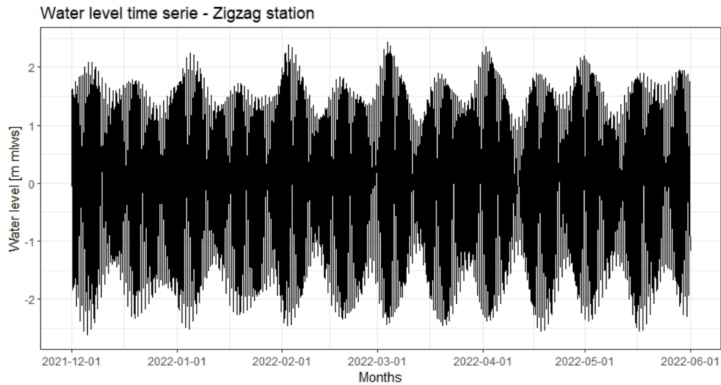
Figure C.1: Water level time series from the Zigzag station. Data measured from 01/12/2021 to 31/05/2022
