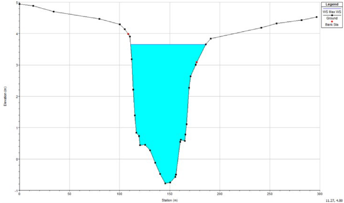
Figure 2.13: Typical cross section configured in the hydrodynamic model
