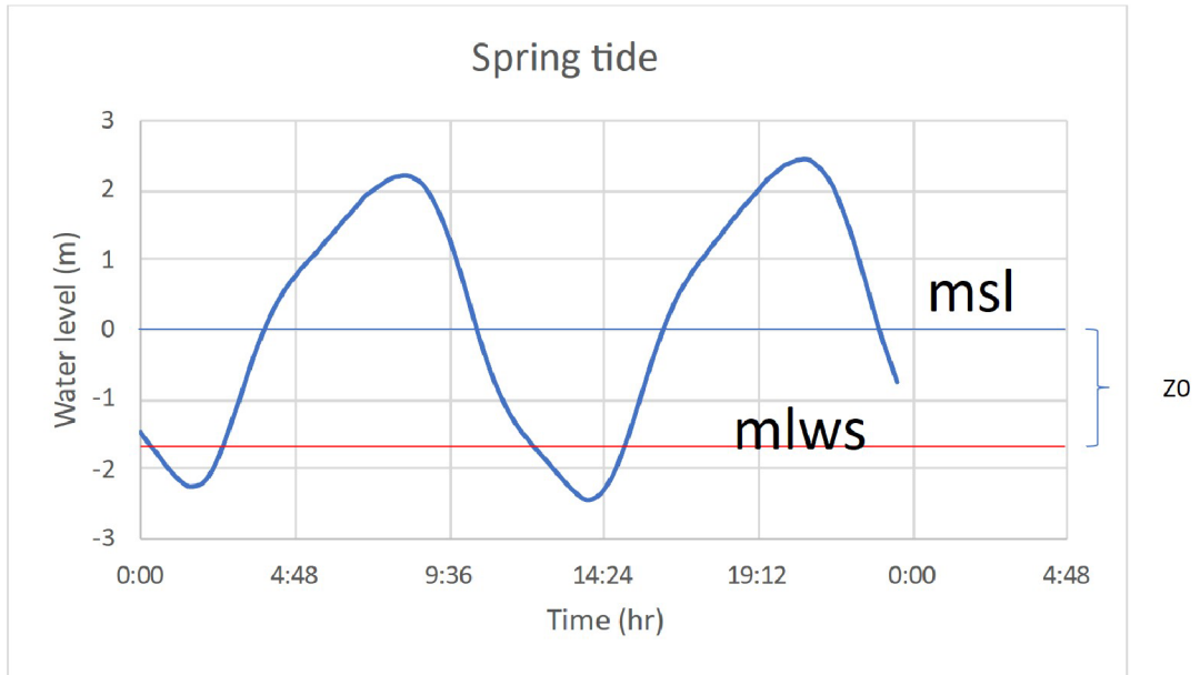
Figure 2.6: Spring tide event registered in Zigzag station. Red line is the mean lowest water surface and blue line is the local mean sea level. Z_0 is the different between msl and mlws.
