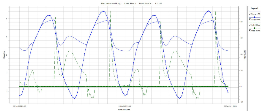
Figure 3.2: Simulation output that represents the stage upstream (blue line) and downstream (blue line with triangles) from gates and total flow through the gates (green line) for increasing tide and decreasing hydrograph.
