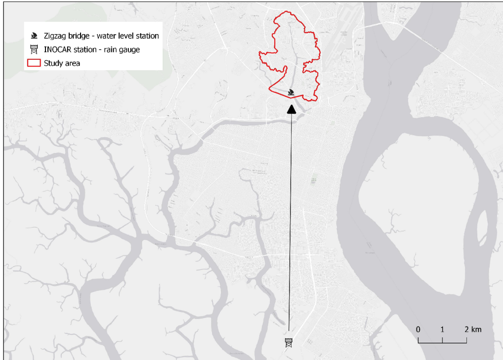
Figure 2.3: Precipitation and tide level stations used in this study
