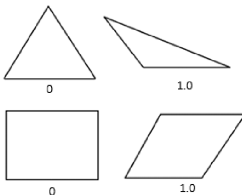
Obr. 45 - Kritérium Skewness
