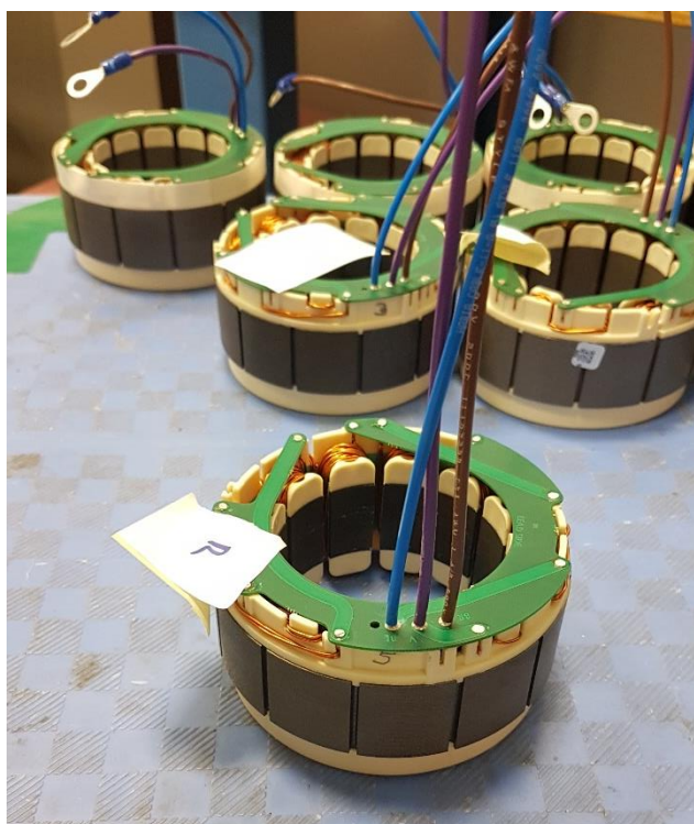
Obr. 7-1 Testované statory
