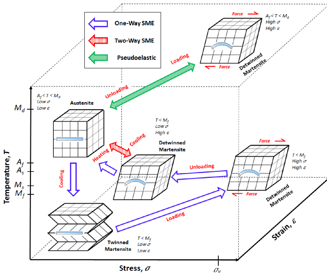
Fig. 2.1. Phase transformation of SMA [1]
