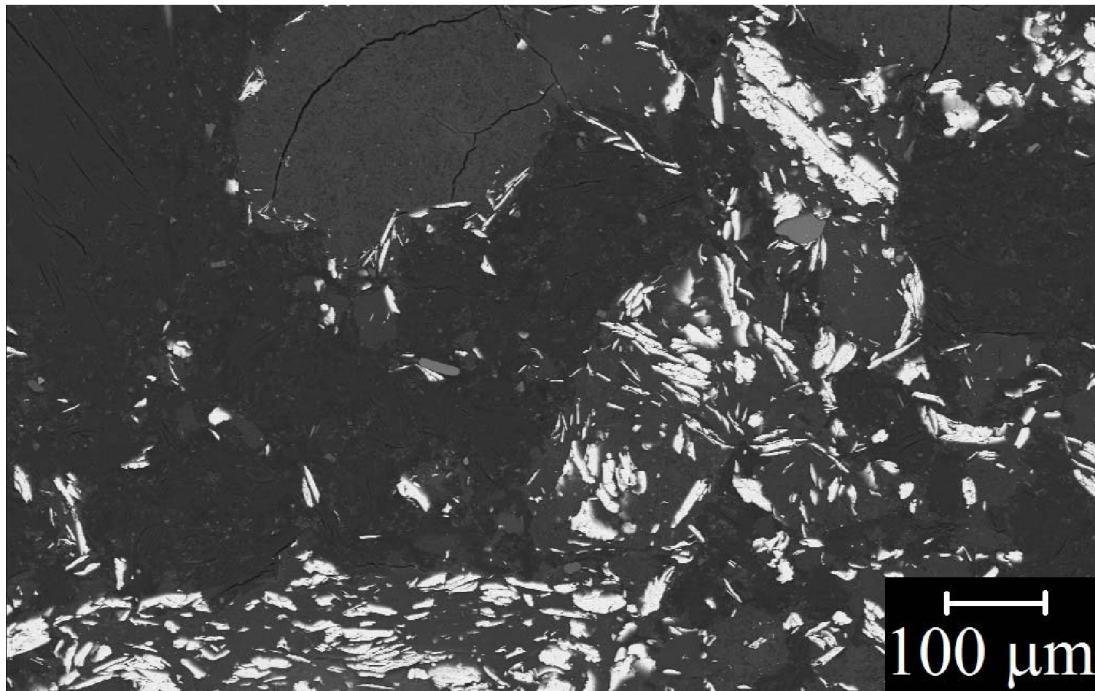
Fig. 3.1 Powder 1 internal structure (cross-section)
