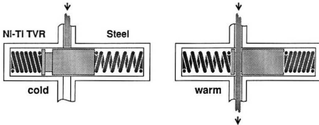
Fig. 2.4 Mercedes-Benz automatic transmission pressure control valve [11]
