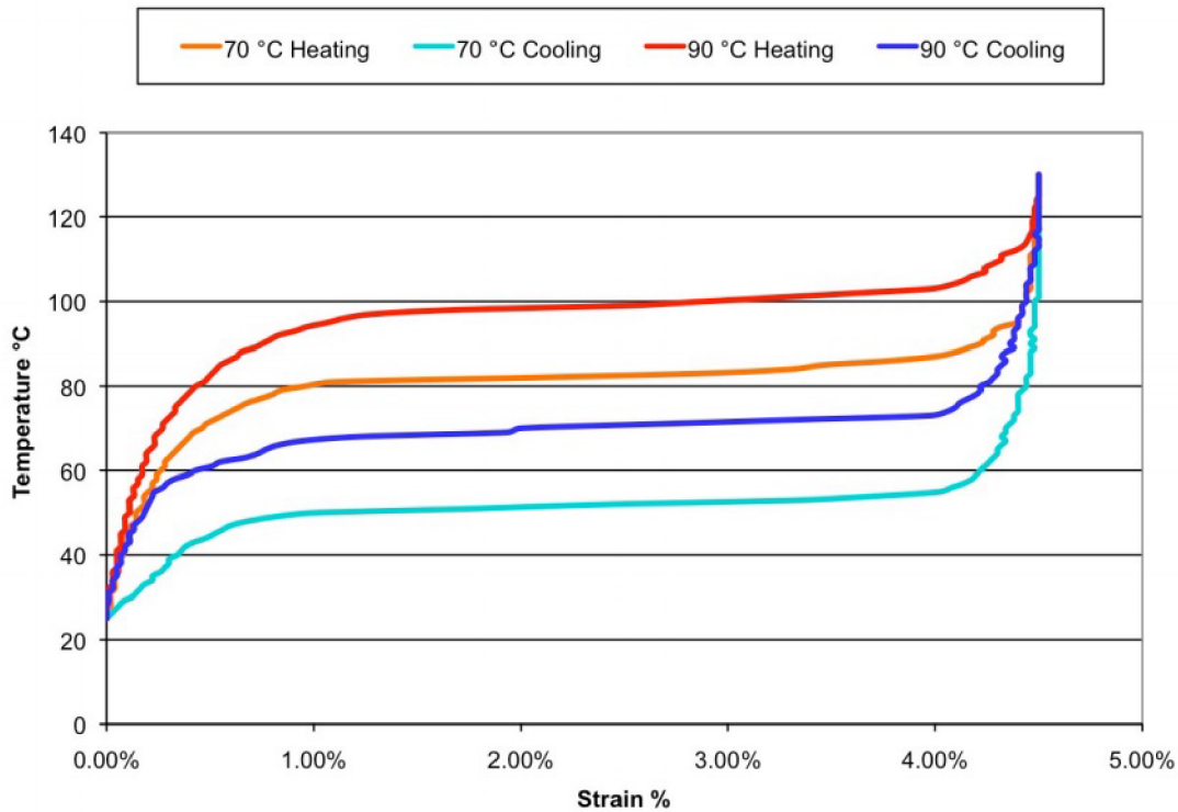
Fig. 2.2 Temperature vs. Strain Characteristics for Dynalloy's "LT" (70°C) and "HT" (90°C) NiTi alloy revealing the effect of hysteresis [7]
