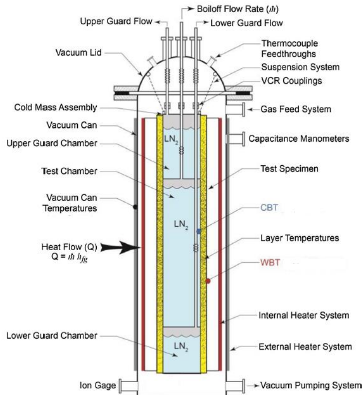
Figure 4-1 Boiloff Calorimeter [30]
