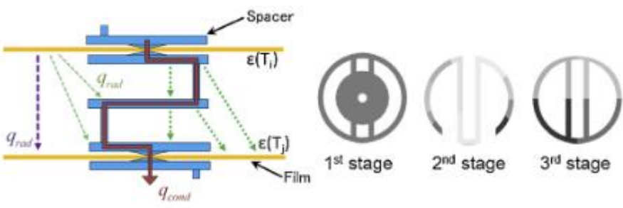
Figure 3-9 Schematics of the heat path and individual stages of the pin [24]
