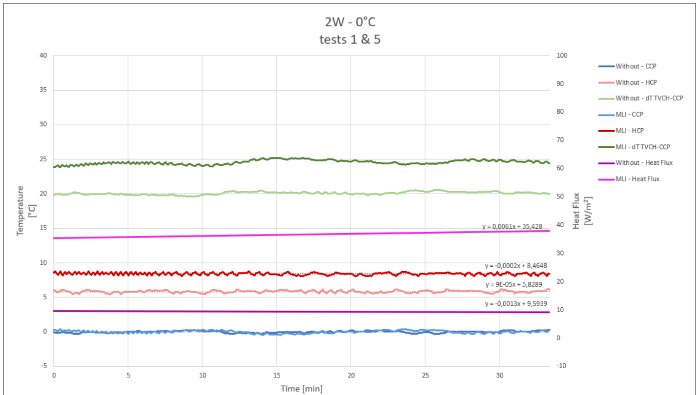
Figure 7-5 Steady-states - tests 1 & 5
