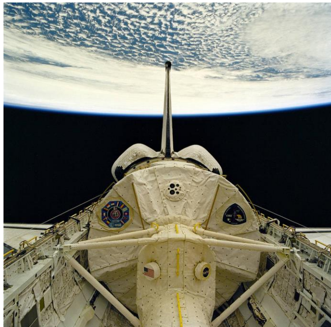
Figure 3-2 Beta Cloth used as an outer cover Atlantis Space Shuttle
