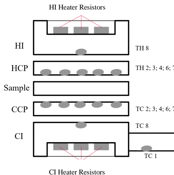
Figure 6-2 Layout of thermocouples and heater resistors
