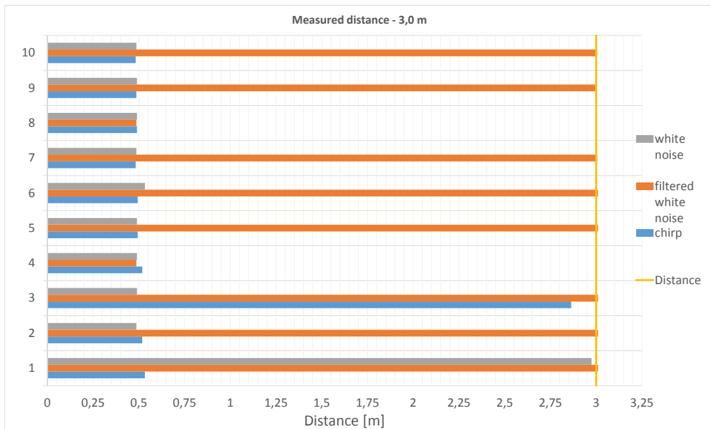
Figure 6.6: Measurement of three meters with chirp, filtered white noise and white noise.
