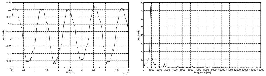
Figure A.5: Recorded signal 880 Hz and its spectrum.
