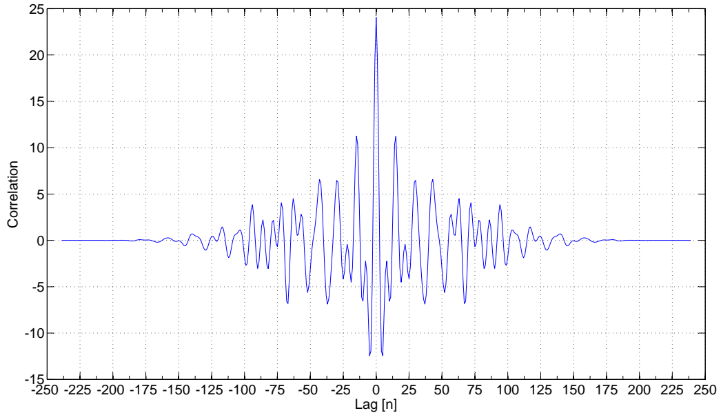
Figure 4.12: Autocorrelation of filtered white noise wave from 4.11.
