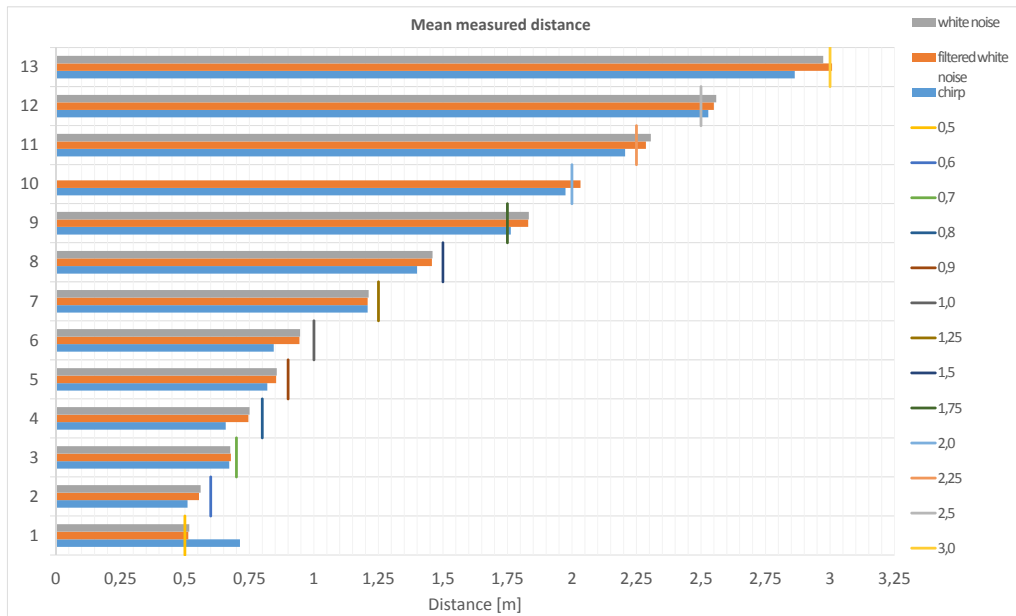
Figure 6.8: Average measured distance for successful cases of chirp, white noise and filtered white noise.
