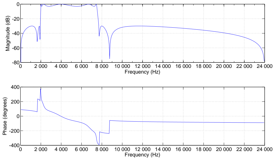
Figure 4.10: Magnitude and phase response of band-pass filter.
