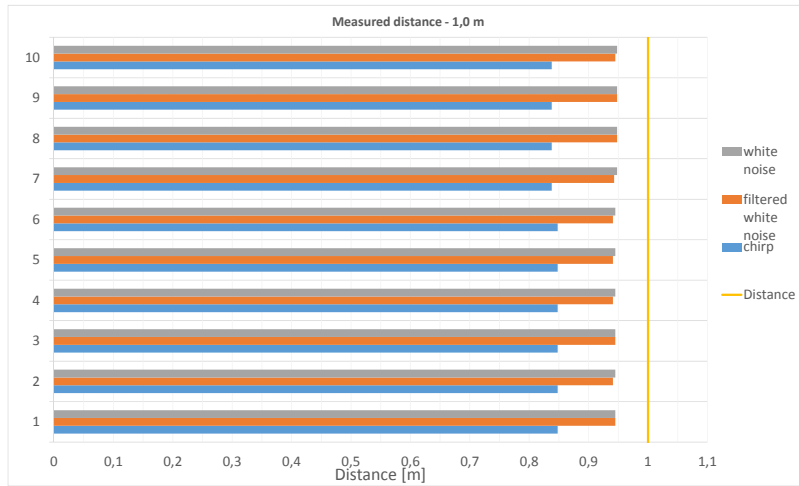
Figure B.6: Measurement of 1.0 meters.
