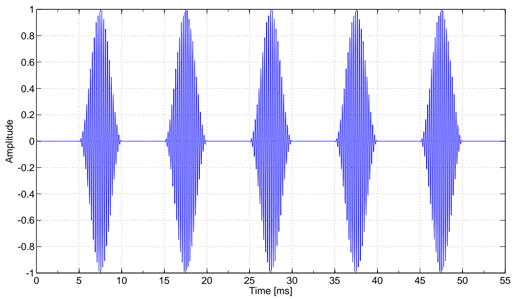
Figure 4.2: Cosine wave 4 500 Hz with repetiton.
