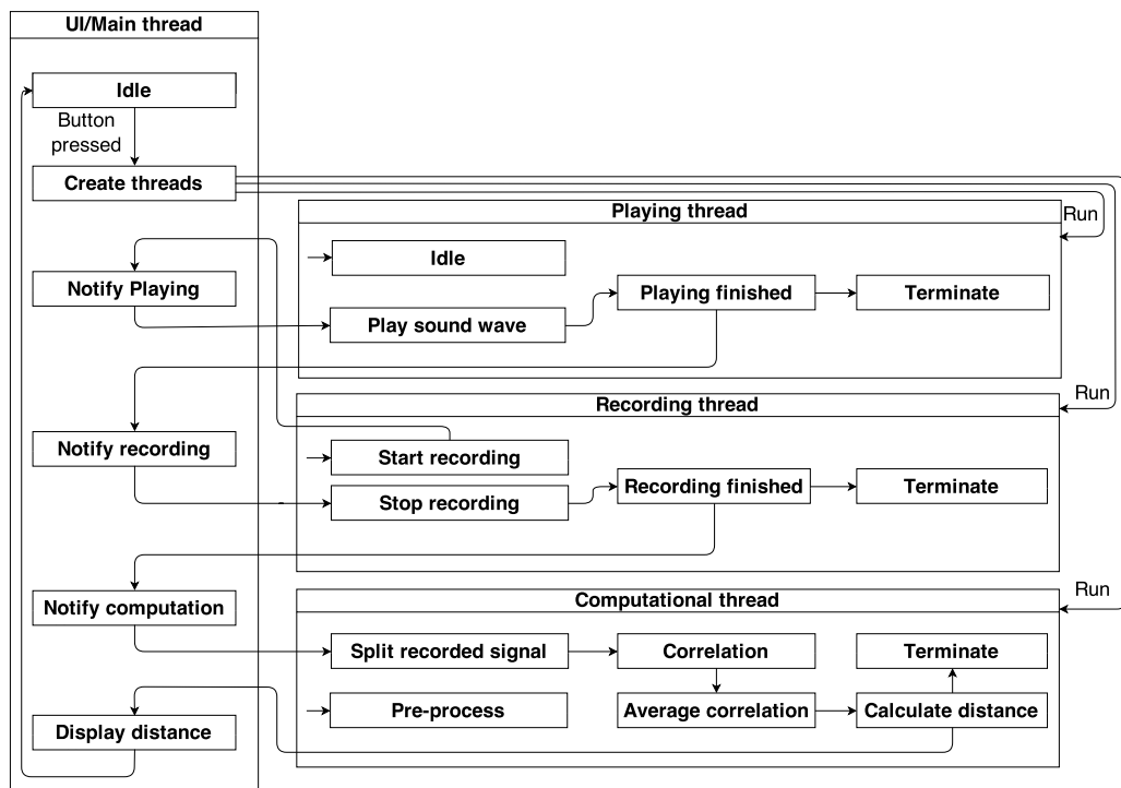
Figure 5.2: Scheme of application functionality and communication between threads.
