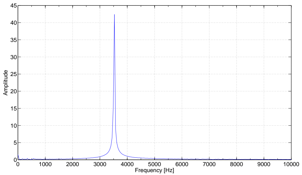
Figure 3.10: Spectrum of sine wave of frequency 3 520 Hz recorded by device.
