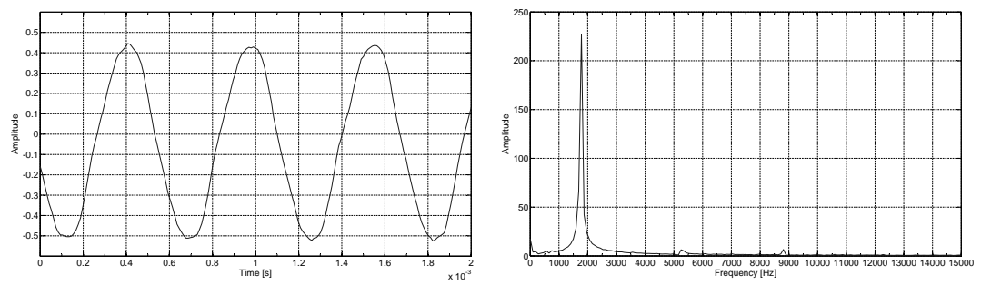
Figure A.6: Recorded signal 1 760 Hz and its spectrum.
