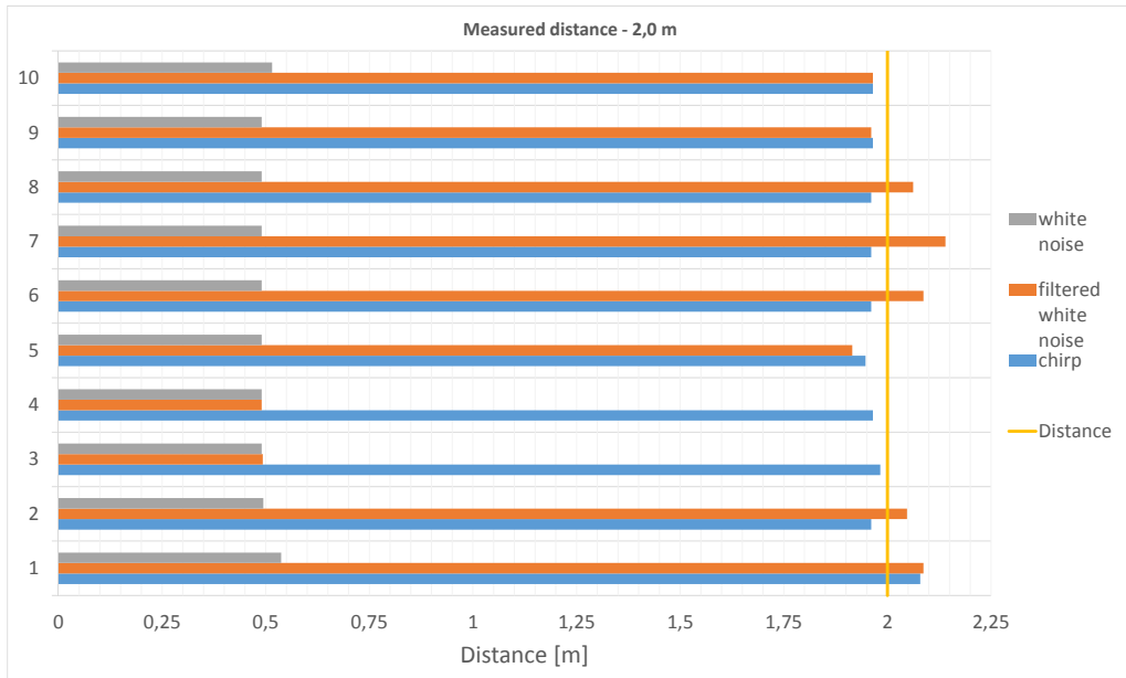
Figure 6.5: Measurement of two meters with chirp, filtered white noise and white noise.
