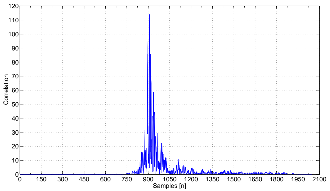
Figure 4.14: Average absolute cross-correlation from figure 4.13.
