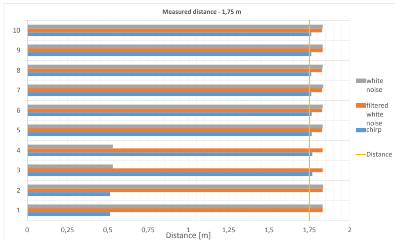
Figure B.9: Measurement of 1.75 meters.
