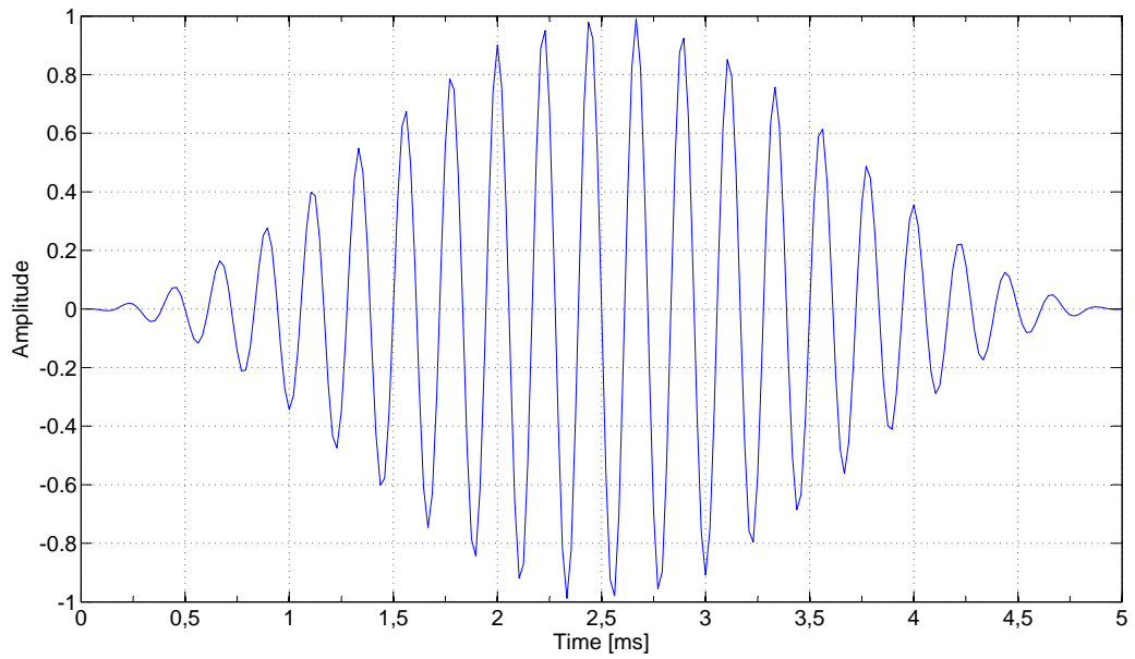
Figure 4.4: Five milliseconds of cosine wave windowed by Hann window.
