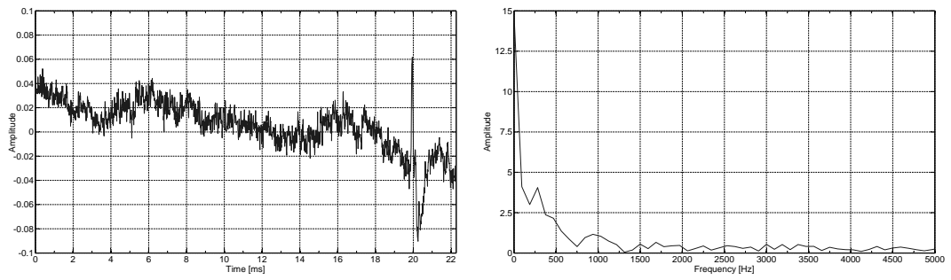
Figure A.3: Recorded signal 220 Hz and its spectrum.
