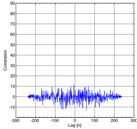
Figure 2.5: Cross-correlation of two independent and random signals.
