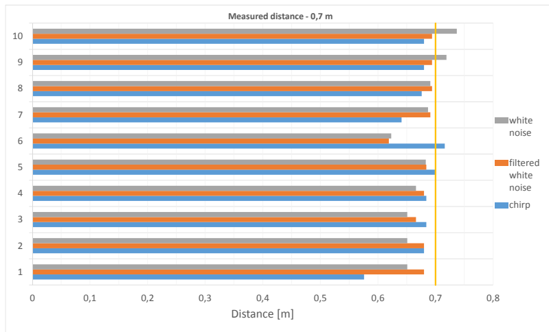
Figure B.3: Measurement of 0.7 meters.
