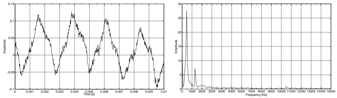
Figure A.4: Recorded signal 440 Hz and its spectrum.
