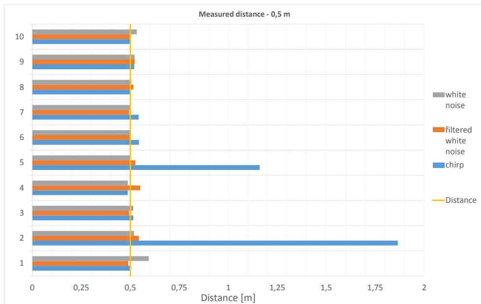
Figure 6.2: Measurement of half meter with chirp, filtered white noise and white noise.
