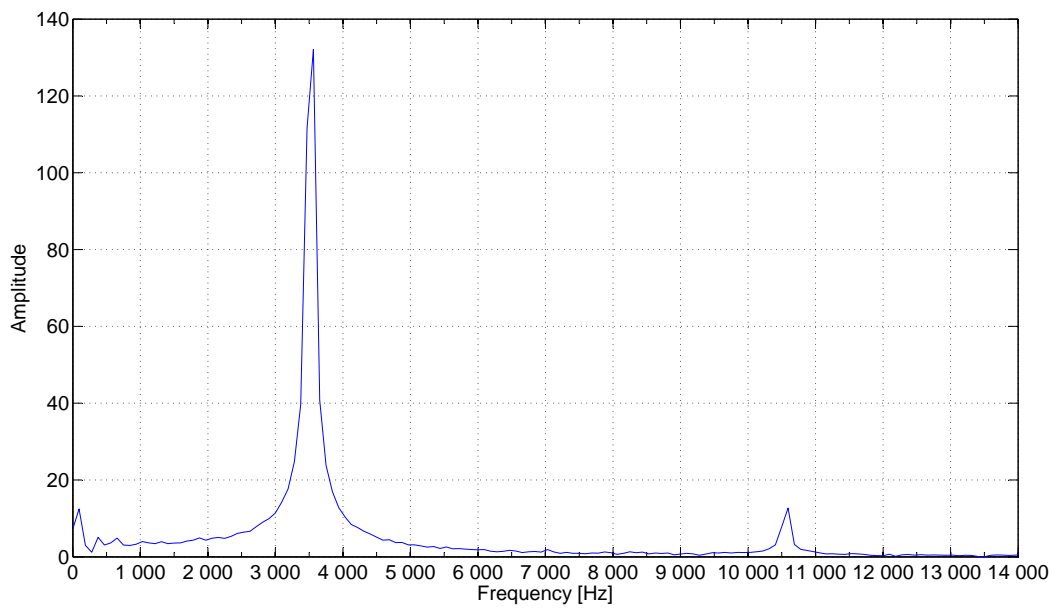
Figure 3.4: Spectrum of sine wave of frequency 3520Hz played by device.
