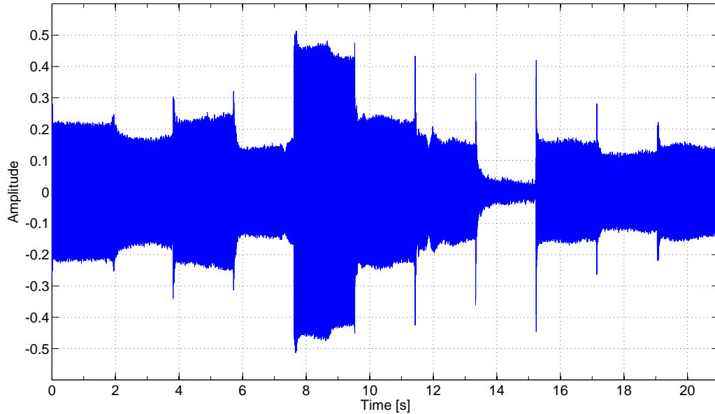
Figure 3.8: Recorded sine waves from 2 000 Hz to 7 000 Hz with step of 500 Hz using optimal volume.
