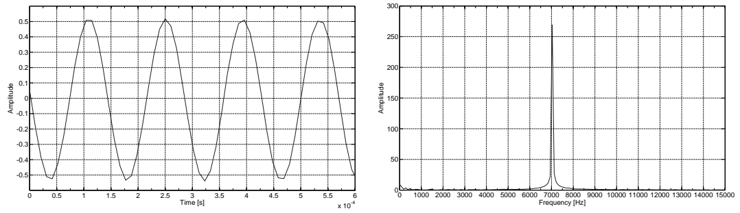
Figure A.8: Recorded signal 7 040 Hz and its spectrum.
