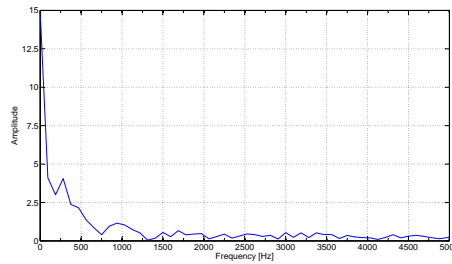
Figure 3.6: Spectrum of sine wave 220 Hz recorded by device.
