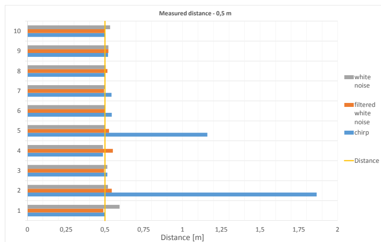
Figure B.1: Measurement of 0.5.
