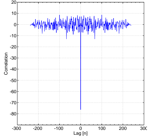
Figure 2.4: Negative auto-correlation.
