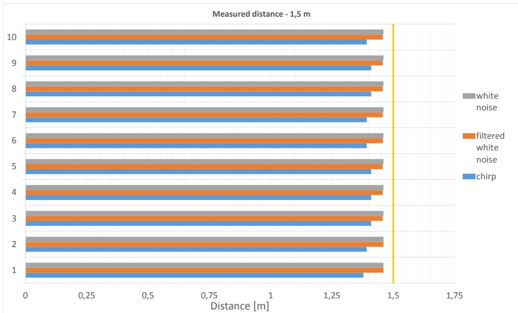
Figure 6.4: Measurement of one and half meter with chirp, filtered white noise and white noise.
