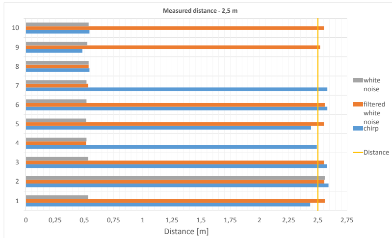
Figure B.12: Measurement of 2.5 meters.
