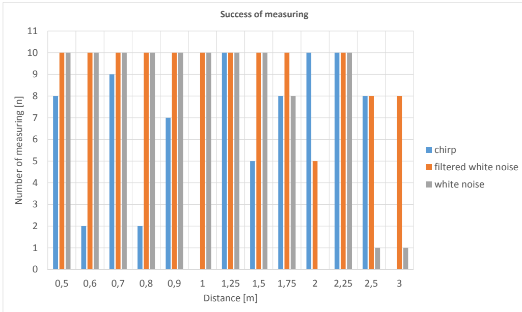
Figure 6.7: Success of measurement for chirp, white noise and filtered white noise.
