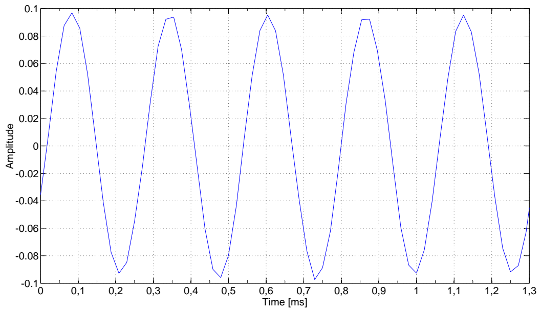
Figure 3.9: Sine wave of frequency 3 520Hz recorded by device.
