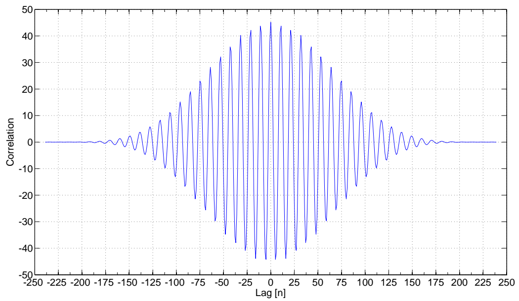
Figure 4.5: Autocorrelation of cosine wave from 4.4.
