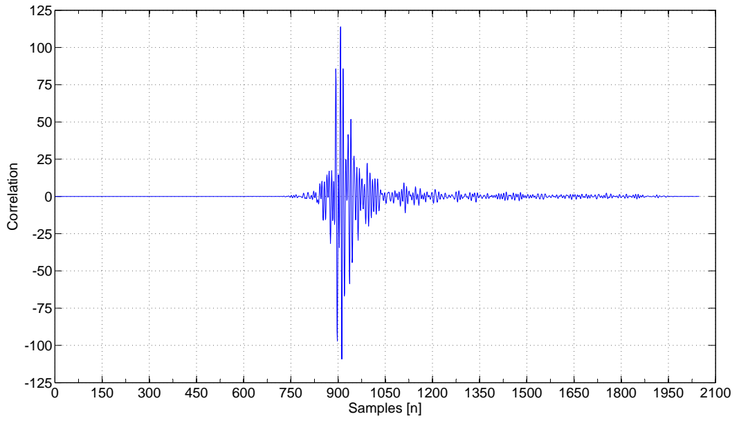
Figure 4.13: Average cross-correlation of filtered white noise.
