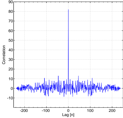
Figure 2.3: Positive auto-correlation.
