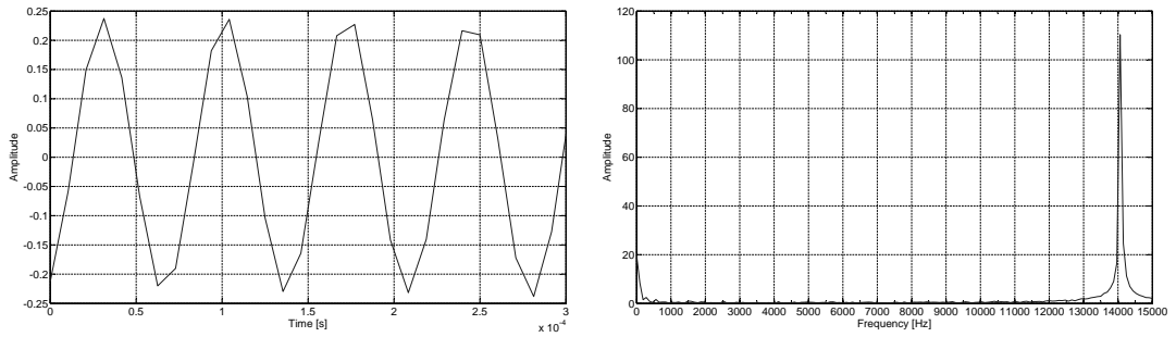
Figure A.9: Recorded signal 14 080 Hz and its spectrum.
