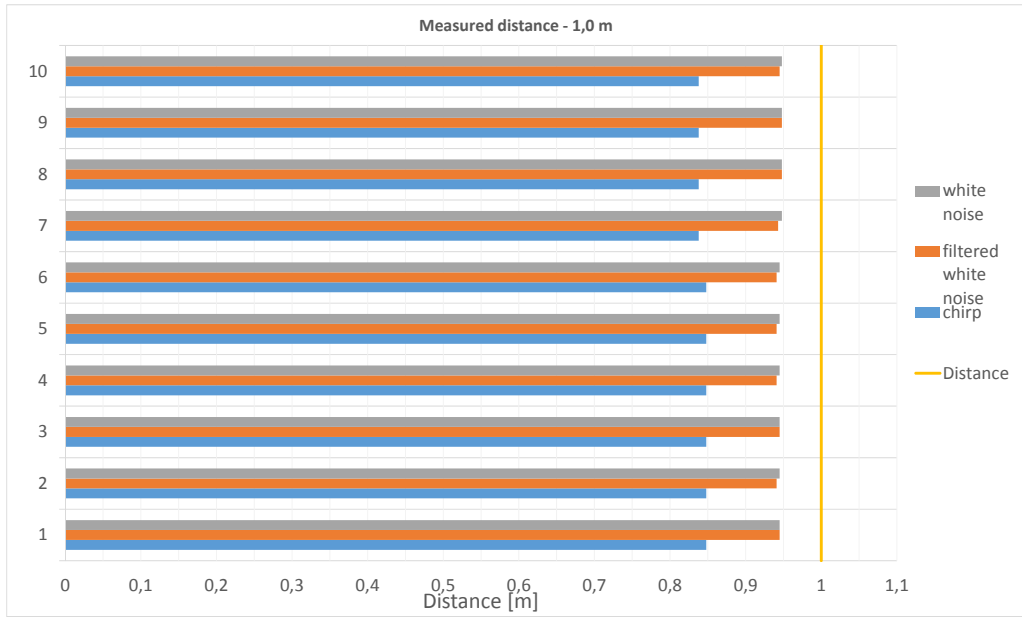
Figure 6.3: Measurement of one meter with chirp, filtered white noise and white noise.
