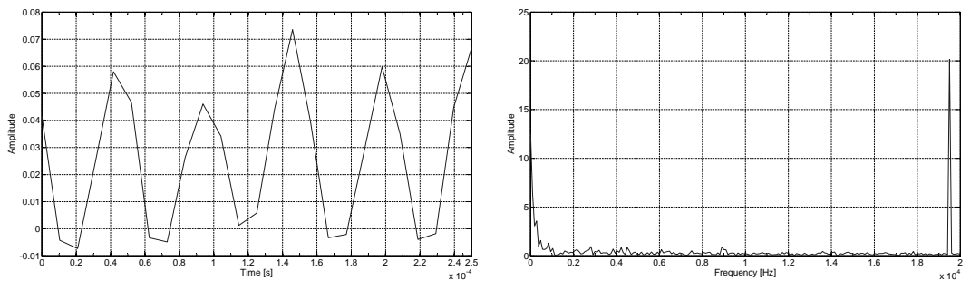
Figure A.10: Recorded signal 19 500 Hz and its spectrum.
