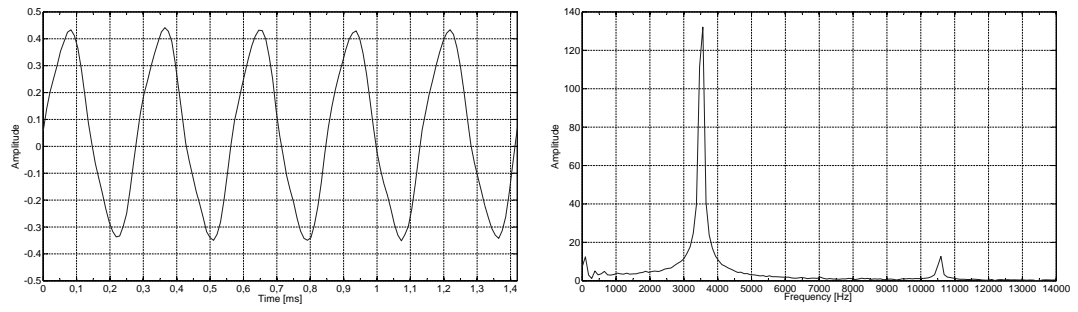
Figure A.7: Recorded signal 3 520 Hz and its spectrum.
