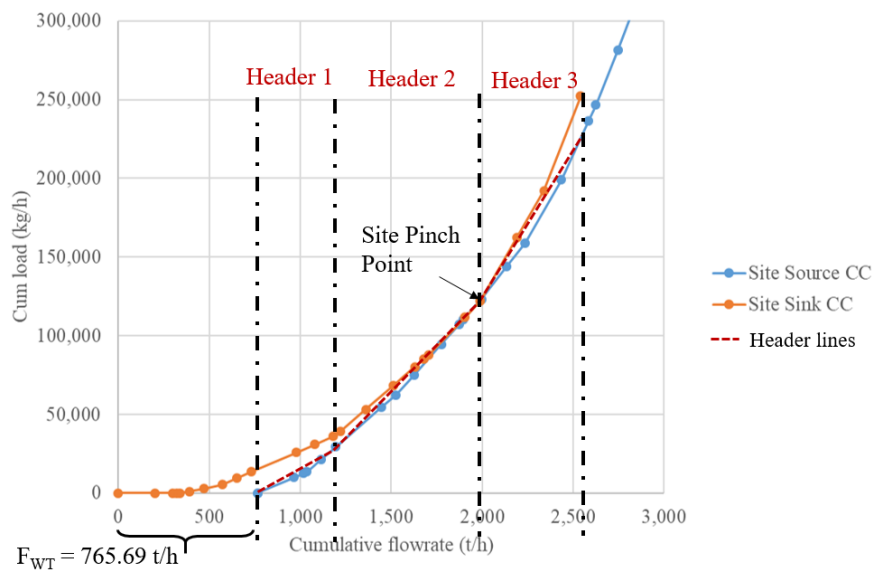
Figure C-1: Total Site water mains design using Composite Curves for a single contaminant case
