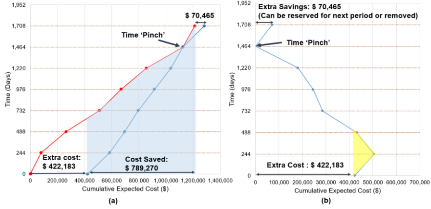
Figure 6-3: Graphical representation of the Pinch Analysis framework after shifting (a) Composite Curves (b) Grand Composite Curve
