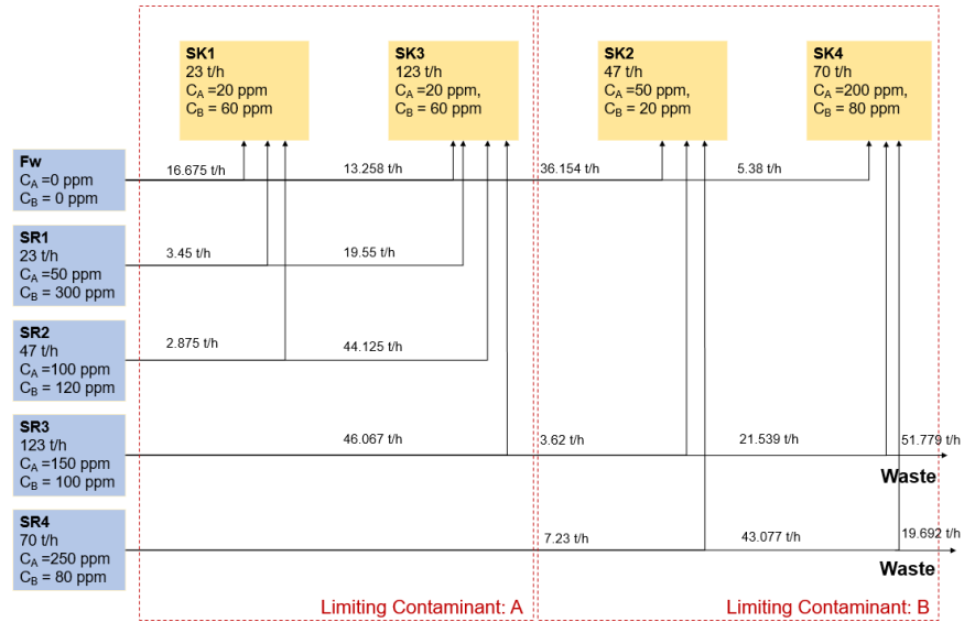
Figure 3-13: Detailed network design for case study 1
