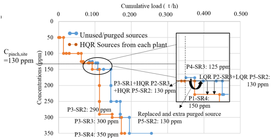
Figure 4-21: Source Transfer Diagram for the case study- 1 st round iteration
