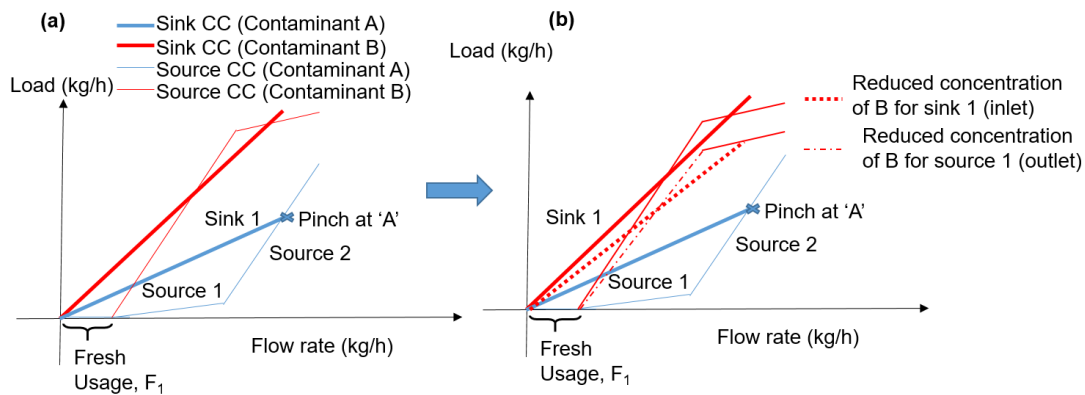
Figure 3-21: Adjusting concentrations of sinks and sources due to the fixed load operation (a) Before adjusting the concentration of sink and source (b) After adjusting the concentration of sink and source
