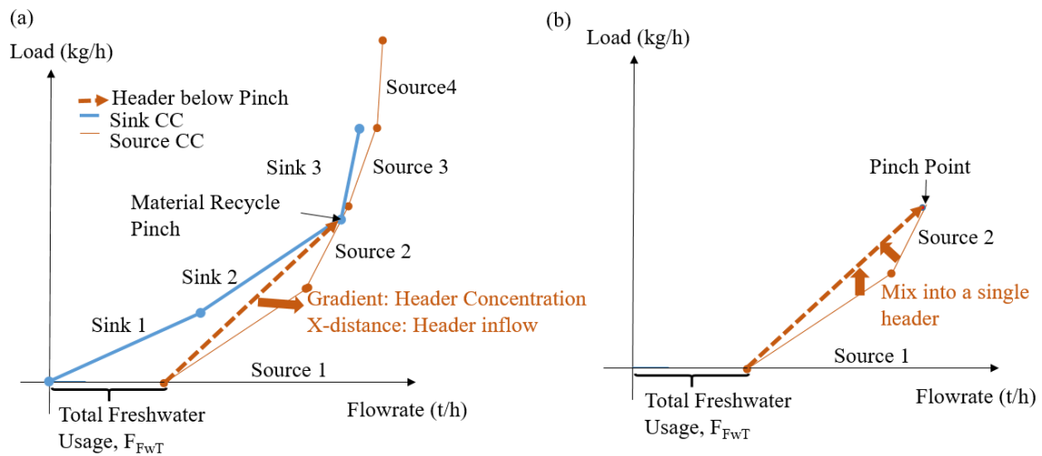
Figure 4-1: Illustrative example of constructing the header line for a single contaminant problem
