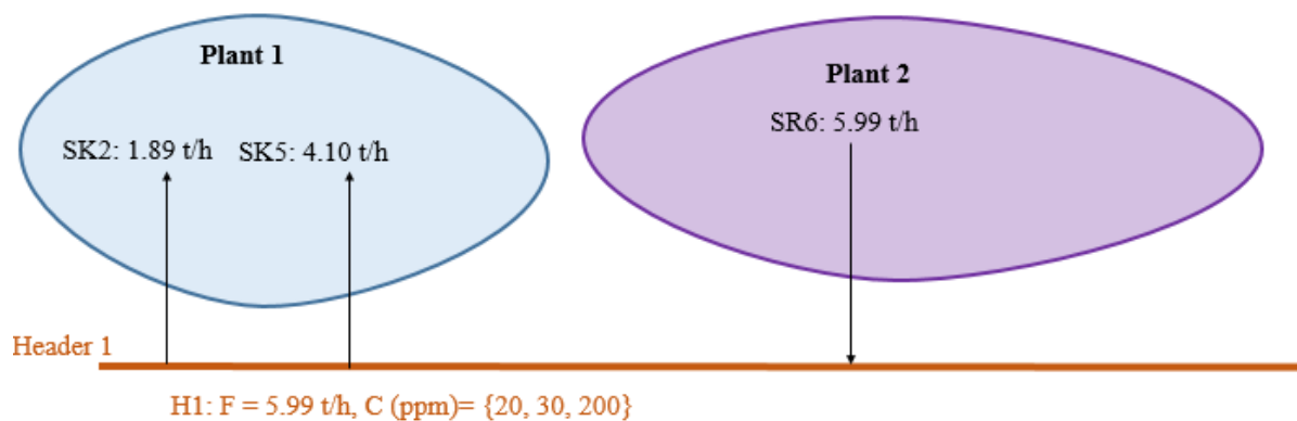
Figure 4-47: Total Site headers allocation for multiple qualities: Two plants study
