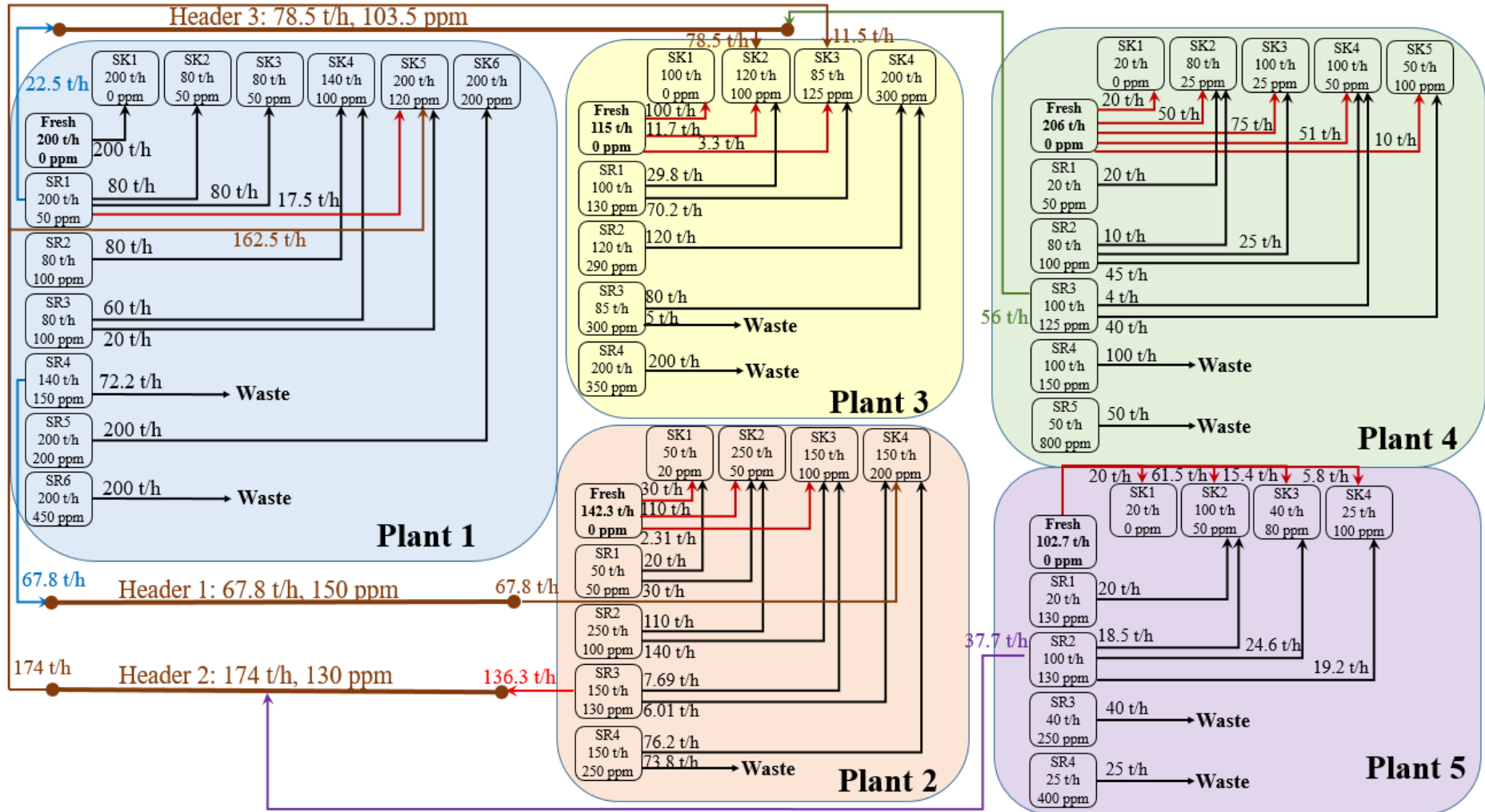
Figure 4-27: Network design for Total Site with three site headers from cross-plant sources. The overall freshwater target is 765.96 t/h with minimal total cross-plant transfer (total flowrates of headers sources) is 320.31 t/h
