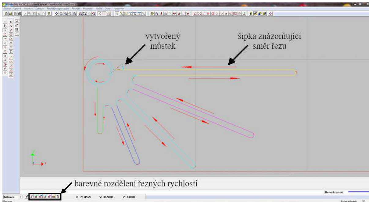
Obr. 40 Software FlowPath.
