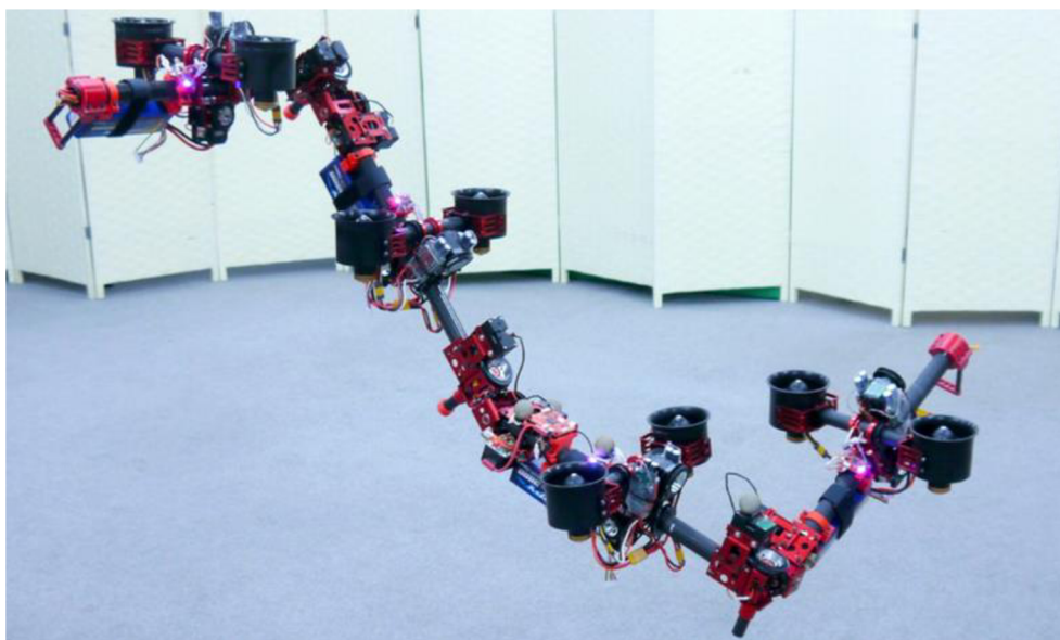
Obr. 6: DRAGON [3]
