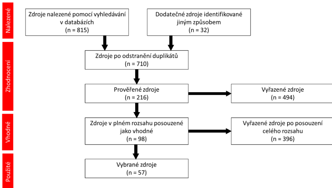
Obr. 2-1 PRISMA diagram
