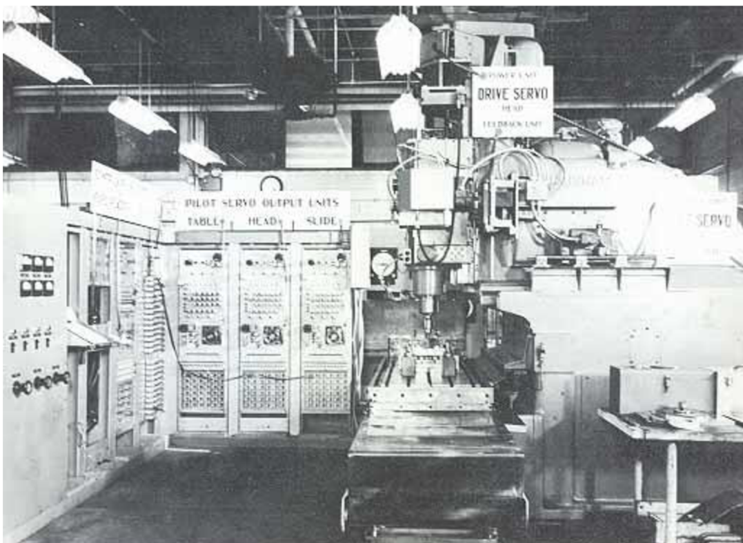
Obr. 2 Frézka Cincinnati Hydro-Tel [42]
