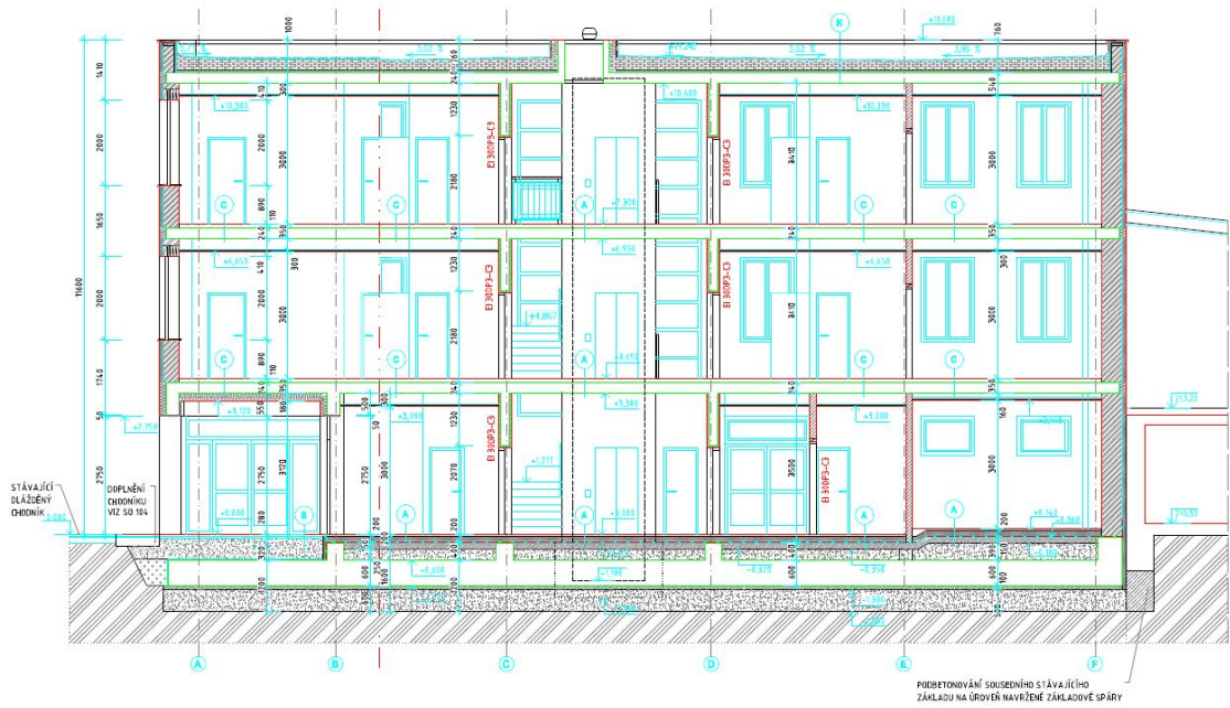
REZ C-C M 1:75
