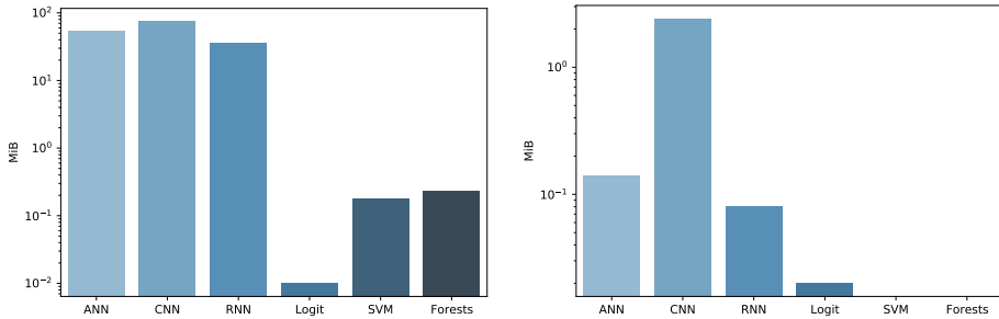
(a) Memory usage when training.
