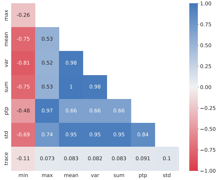
Figure 3.2: Correlation of features
