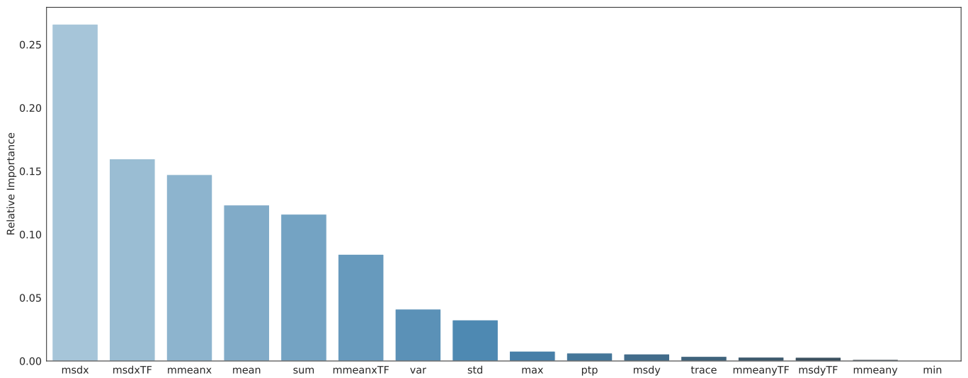
Figure 3.13: Random forest's feature importances.
