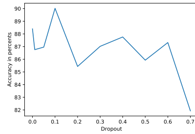
(b) Accuracy per dropout value in hidden layer using 200 neurons in hidden layer.
