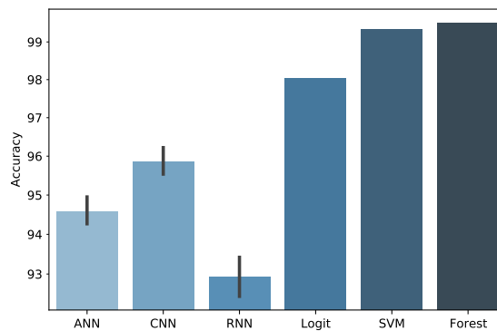
Figure 4.4: Prototype accuracies
