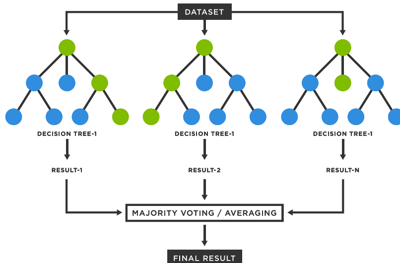
Figure 2.9: Random forests scheme taken from [3]
