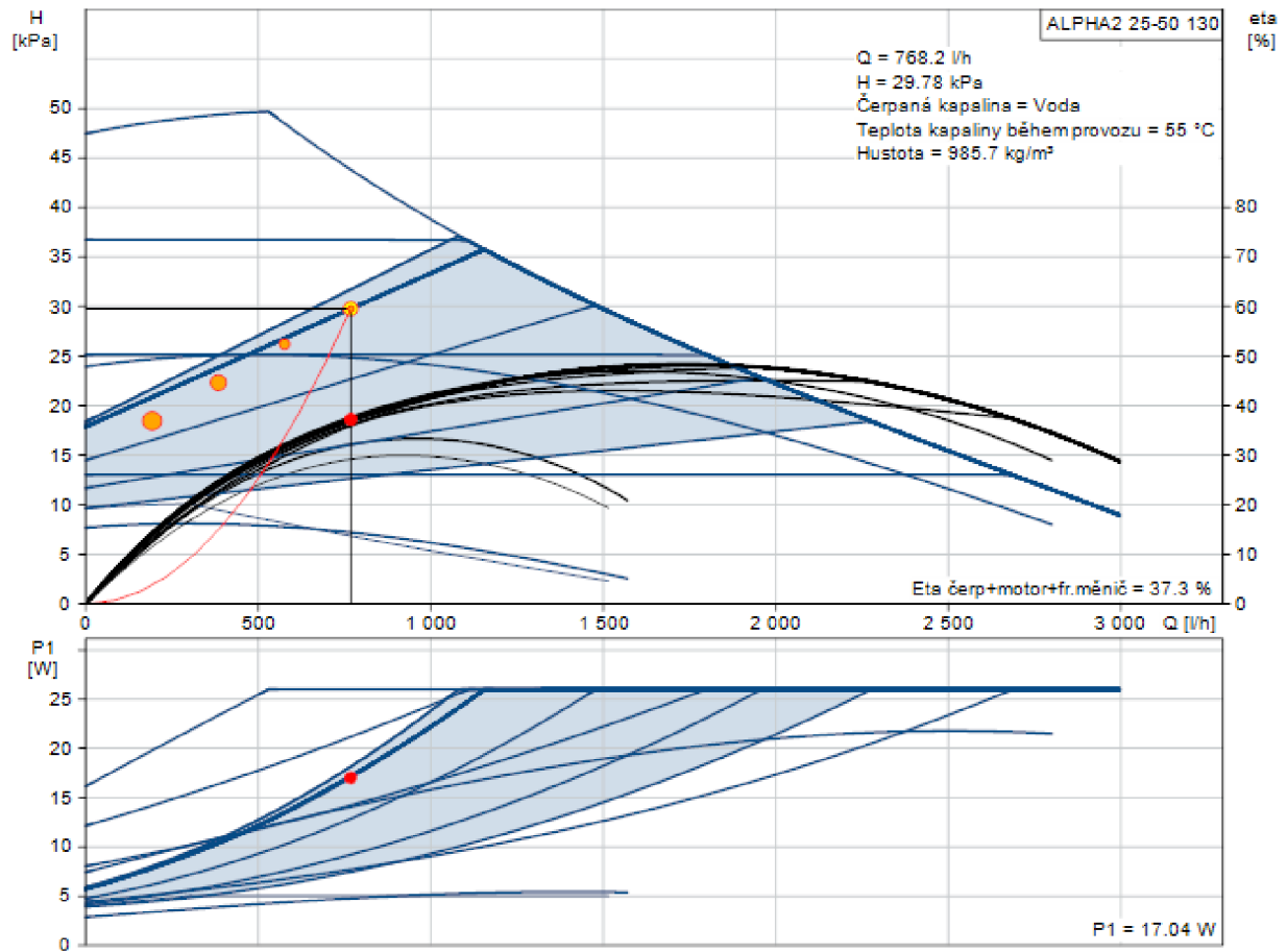
Figure 52-circulating pump Grundfos ALPHA A2 25-50 130 [57]
