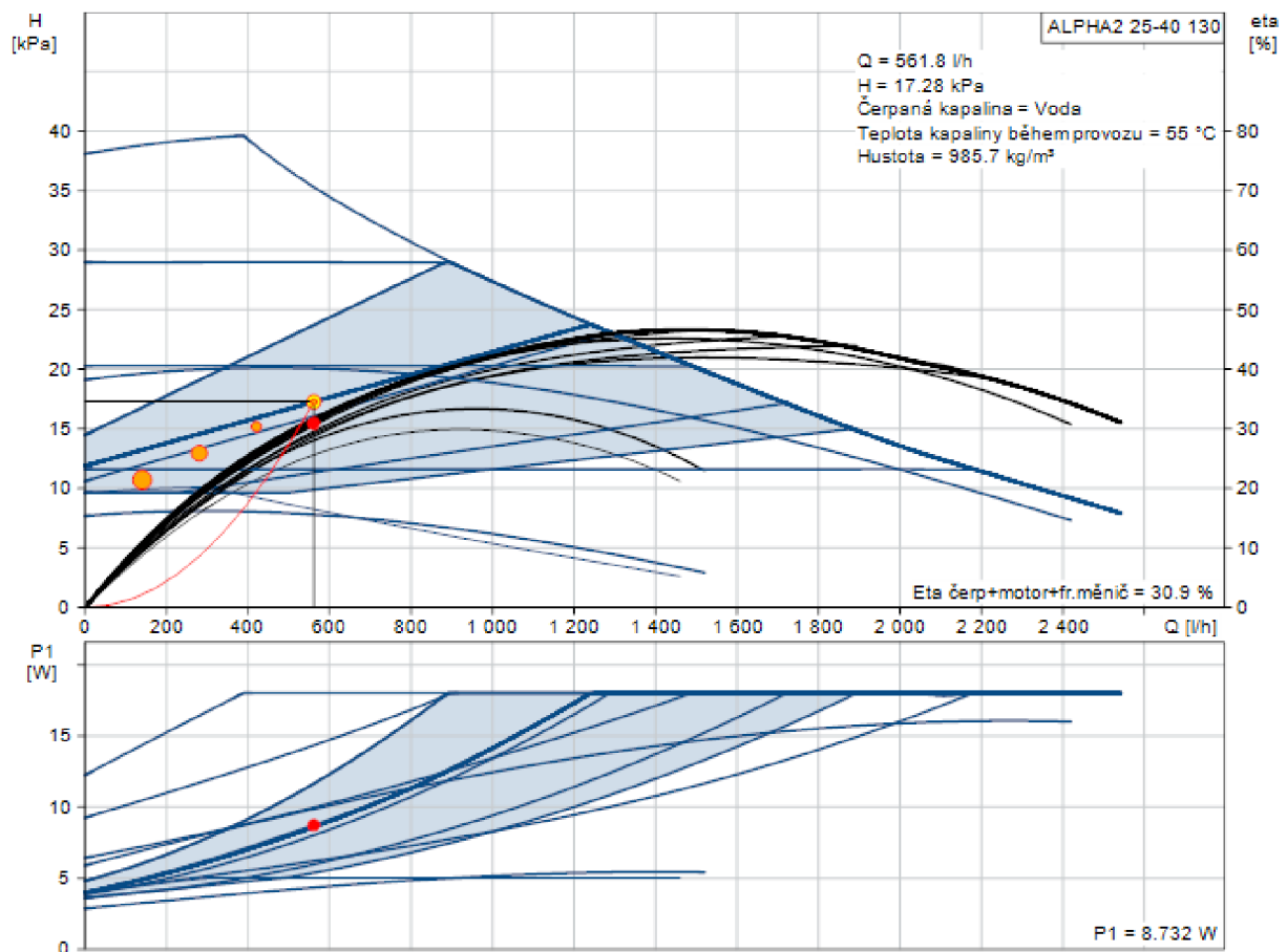
Figure 55-circulating pump Grundfos ALPHA A2 25-40 130[57]
