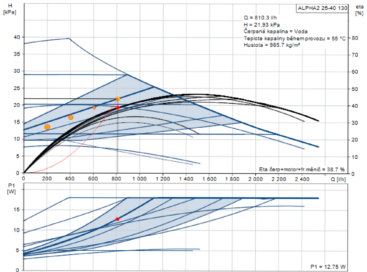
Figure 53-circulating pump Grundfos ALPHA A2 25-40 130[57]
