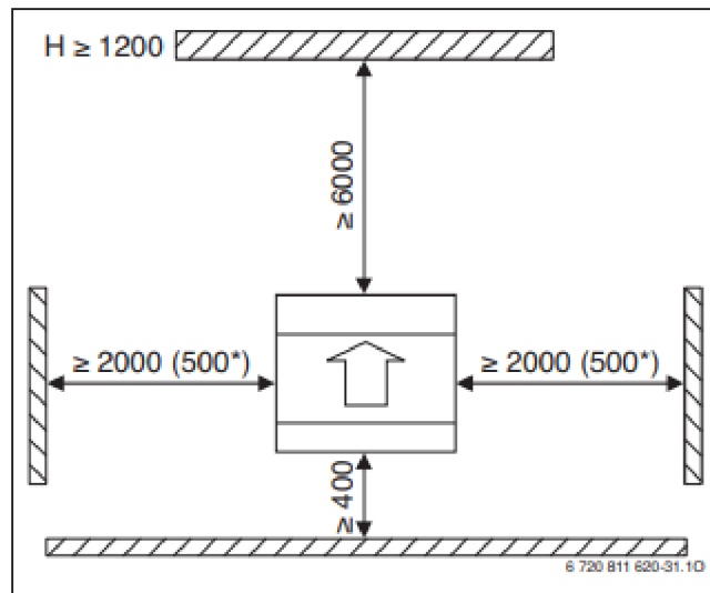
Figure 36- minimal distance around heat pump[40]
