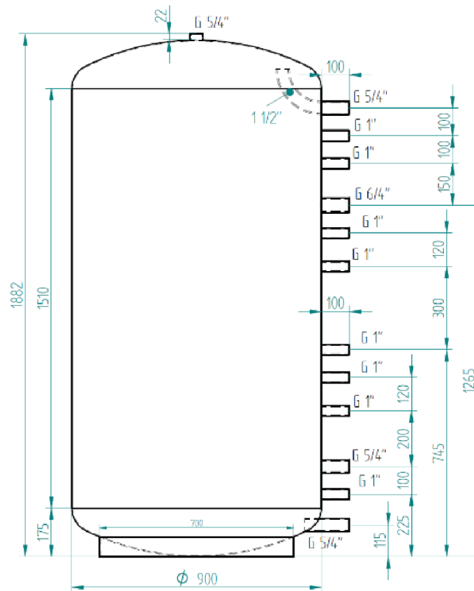
Figure 33-storage tank LMG 1200 0V [47]
