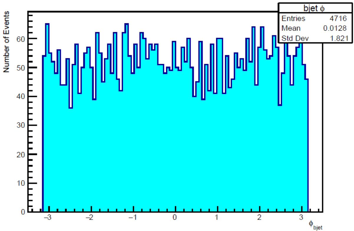
Figure 12: Histogram of the \phi of b jets in the top-quark enriched sample from ATLAS p-Pb collisions.
