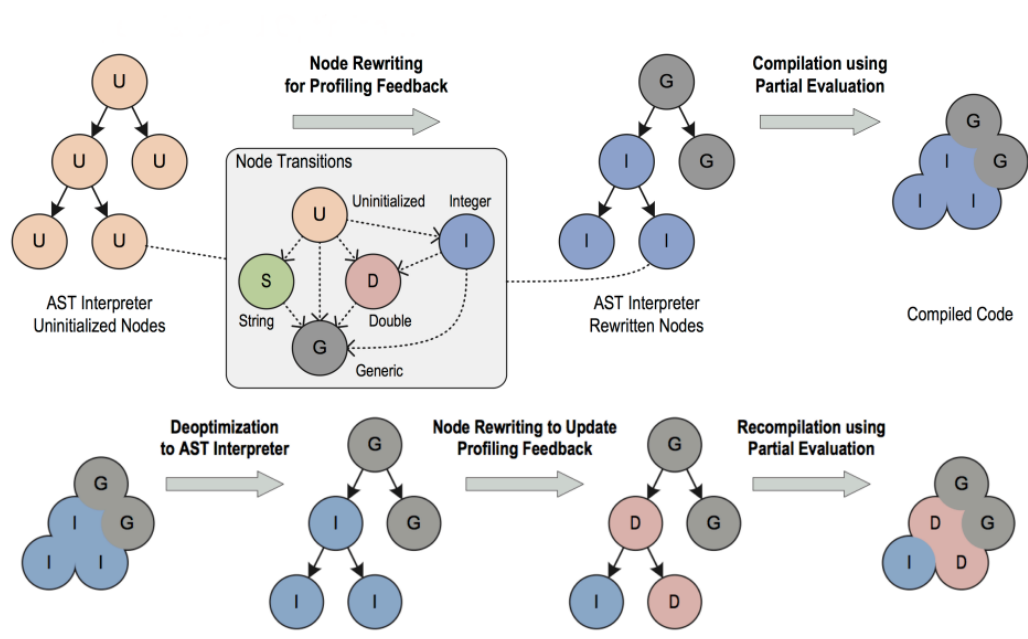
Figure 4.6: Node optimization and deoptimization in Truffle 6
