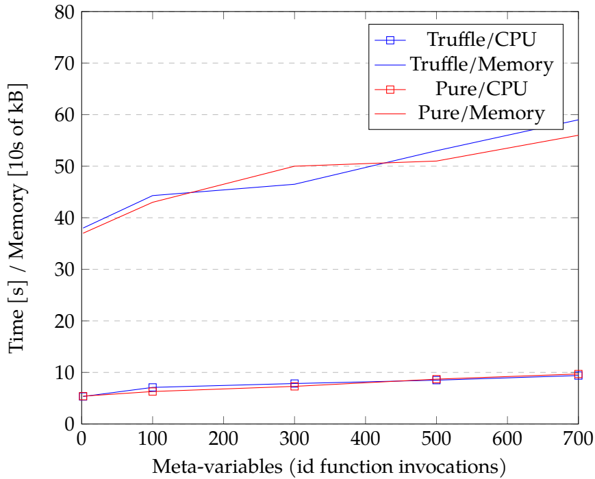
Figure 5.3: Results of evaluation on the id stress test
