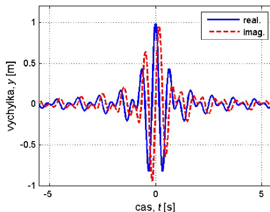
Obr. 1.11: Shannonova vlnka 1-1
