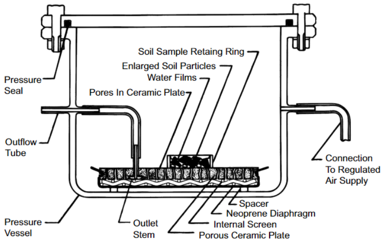
Fig. 18. Cross section of the pressure vessel (Soilmoisture, 2008).
