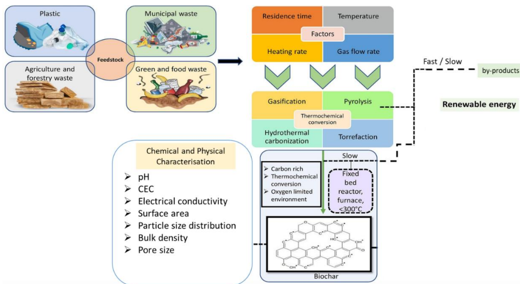
Fig. 10. Different source material and thermochemical methods to convert biomass/waste to biochar. various activation and characterization techniques are also schematically summarized (modified from Uday et al., 2022).
