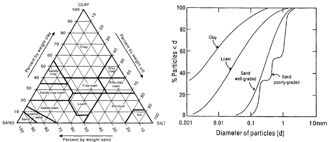
Fig. 4. Left) The conventional textural triangle to classify the soils regarding their texture. Right) various soil material particle size distribution curves (Hillel, 1980)
