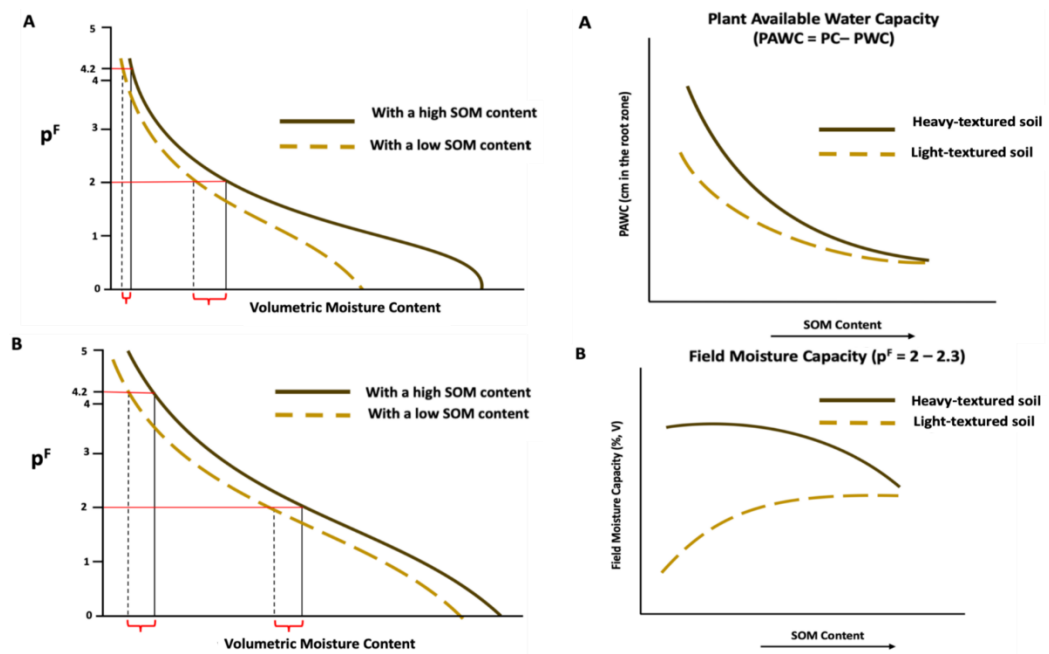
Fig. 7. A schematic of pF curve in soils, showing different cases of OM application responses (Lal, 2020)
