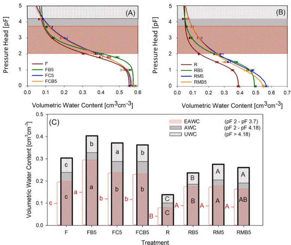
Fig. 21. Water Retention Curves of Fluvisol (A) and Regosol (B) experiments, and division of soil water into unavailable (UWC) and available (AWC). The part of easy-available for plant (EAWC) is red-marked (C). Individual figures (top) show water retention curves of Regosol and Fluvisol samples (non)enriched by organic amendments. Means of 6 replicates are highlighted by bullets. The graphs are supported by the more detailed at Table S3 (standard deviation and letter differences are presented). Different letters in figure (C) represent statistical differences between variants by Tukey HSD for each trial (capitals for trial T2), (Seyedsadr et al., 2021).
