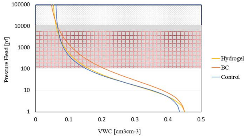
Fig. 26. Water Retention Curves of biochar and hydrogel experiment in Cambisol.
