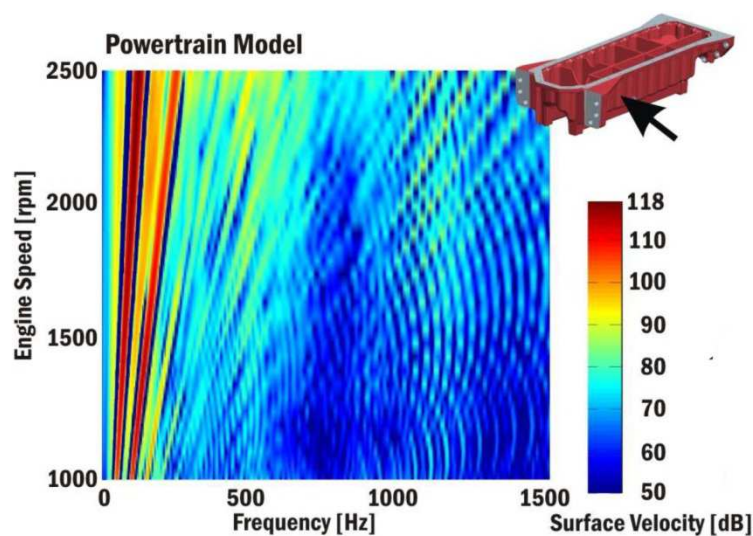
Figure 12 Campbell diagram [1]
