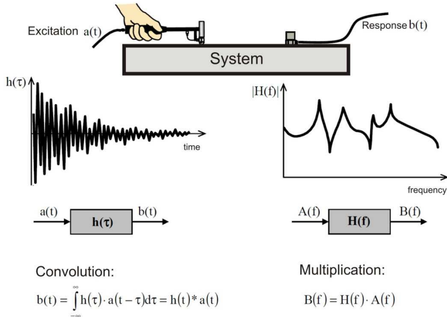
Figure 38 Frequency response function and impulse response function [24]
