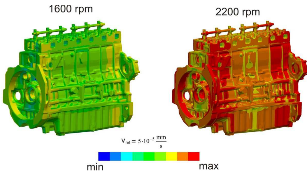
Figure 69 Surface noise level
