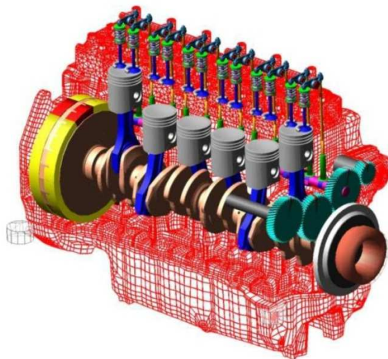
Figure. 10 MBS model[1]
