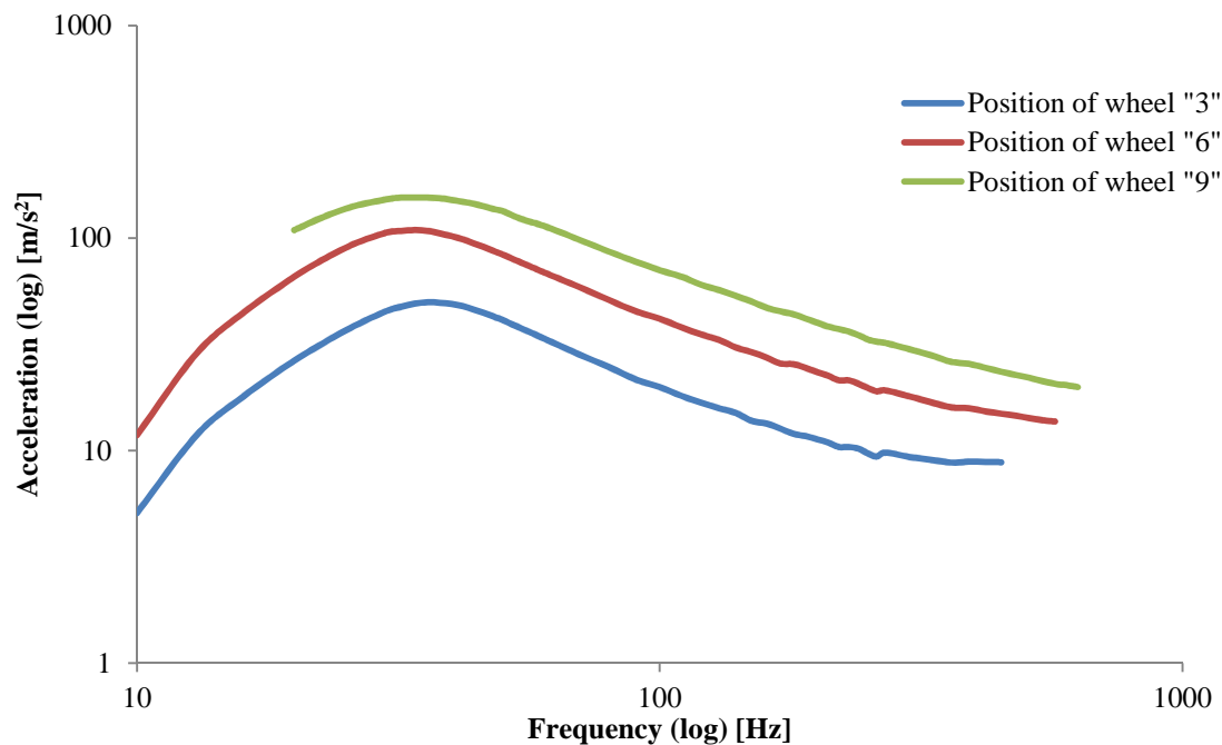
Figure 31 Graph acceleration for exciter
