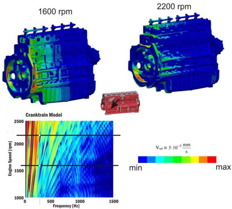
Figure 67 Mobility for 250 Hz
