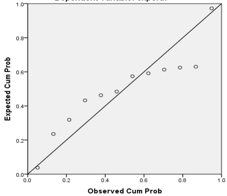
Normal P-P Plot of Regression Standardized Residual Dependent Variable: exportx
